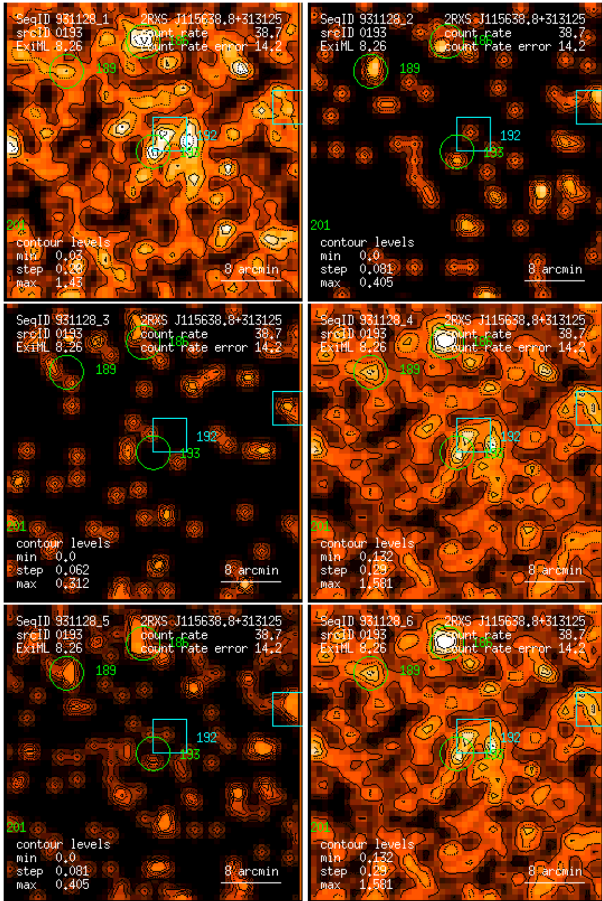
Figure 193: RASS 931128: detection 0193: band rate images, Gaussian filter: (1) PSPC channels 11 – 41, (2) 52 – 90, (3) 91 – 201, (4) 11 – 235, (5) 52 – 201, (6) 11 – 201. Broad band rates in counts/ks. Band rate contour levels in counts/ks/arcmin 2 .
