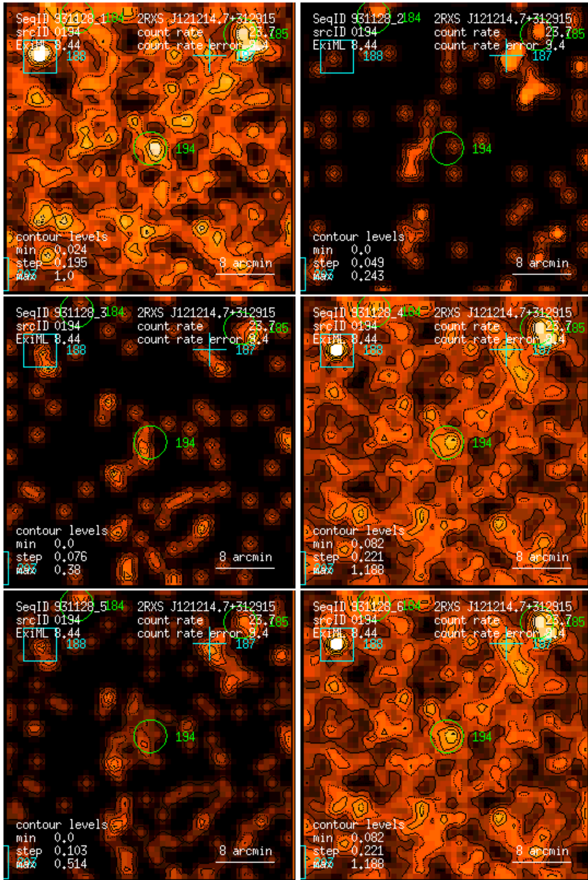
Figure 194: RASS 931128: detection 0194: band rate images, Gaussian filter: (1) PSPC channels 11 – 41, (2) 52 – 90, (3) 91 – 201, (4) 11 – 235, (5) 52 – 201, (6) 11 – 201. Broad band rates in counts/ks. Band rate contour levels in counts/ks/arcmin 2 .
