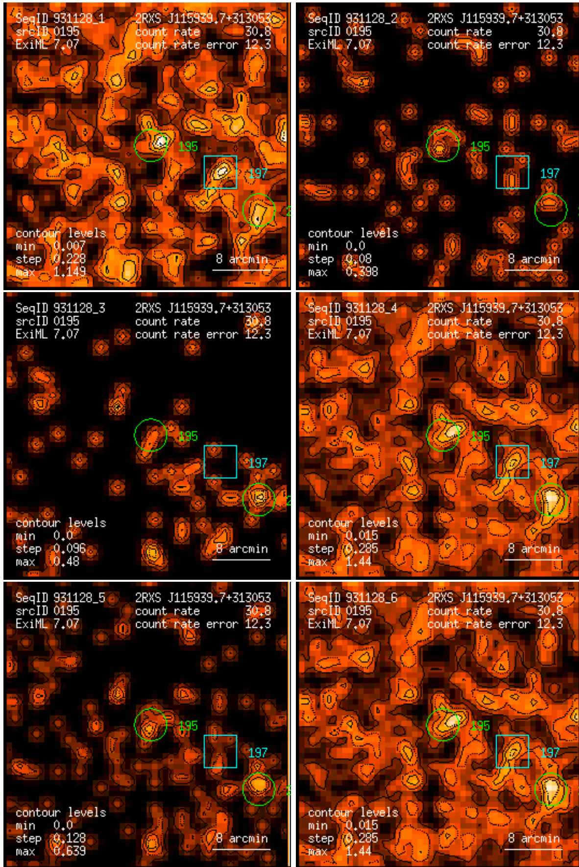
Figure 195: RASS 931128: detection 0195: band rate images, Gaussian filter: (1) PSPC channels 11 – 41, (2) 52 – 90, (3) 91 – 201, (4) 11 – 235, (5) 52 – 201, (6) 11 – 201. Broad band rates in counts/ks. Band rate contour levels in counts/ks/arcmin 2 .
