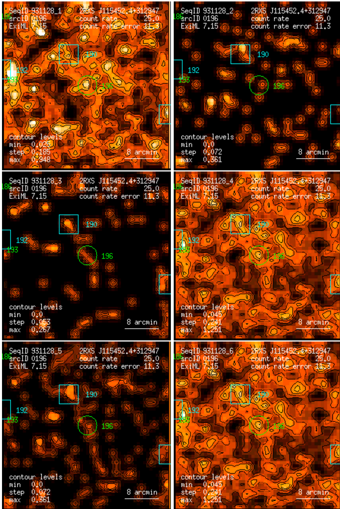
Figure 196: RASS 931128: detection 0196: band rate images, Gaussian filter: (1) PSPC channels 11 – 41, (2) 52 – 90, (3) 91 – 201, (4) 11 – 235, (5) 52 – 201, (6) 11 – 201. Broad band rates in counts/ks. Band rate contour levels in counts/ks/arcmin 2 .
