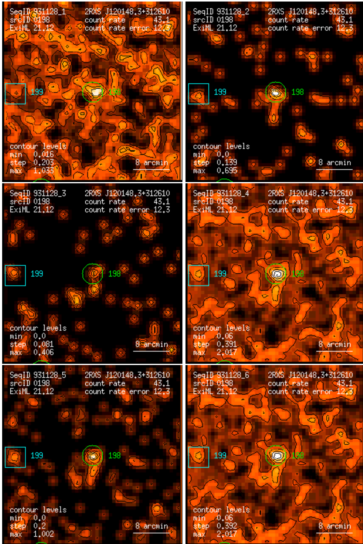
Figure 198: RASS 931128: detection 0198: band rate images, Gaussian filter: (1) PSPC channels 11 – 41, (2) 52 – 90, (3) 91 – 201, (4) 11 – 235, (5) 52 – 201, (6) 11 – 201. Broad band rates in counts/ks. Band rate contour levels in counts/ks/arcmin 2 .
