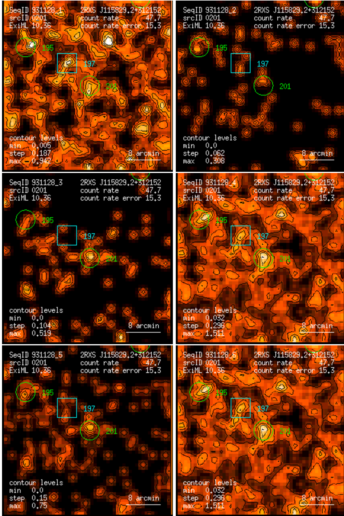
Figure 201: RASS 931128: detection 0201: band rate images, Gaussian filter: (1) PSPC channels 11 – 41, (2) 52 – 90, (3) 91 – 201, (4) 11 – 235, (5) 52 – 201, (6) 11 – 201. Broad band rates in counts/ks. Band rate contour levels in counts/ks/arcmin 2 .
