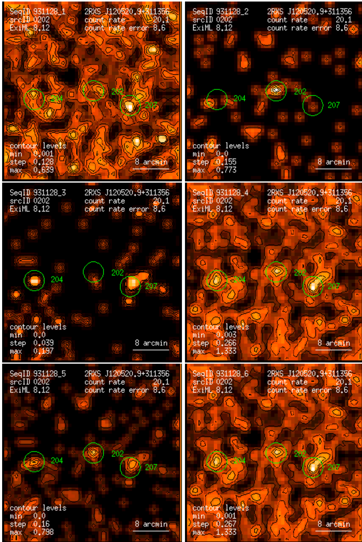
Figure 202: RASS 931128: detection 0202: band rate images, Gaussian filter: (1) PSPC channels 11 – 41, (2) 52 – 90, (3) 91 – 201, (4) 11 – 235, (5) 52 – 201, (6) 11 – 201. Broad band rates in counts/ks. Band rate contour levels in counts/ks/arcmin 2 .
