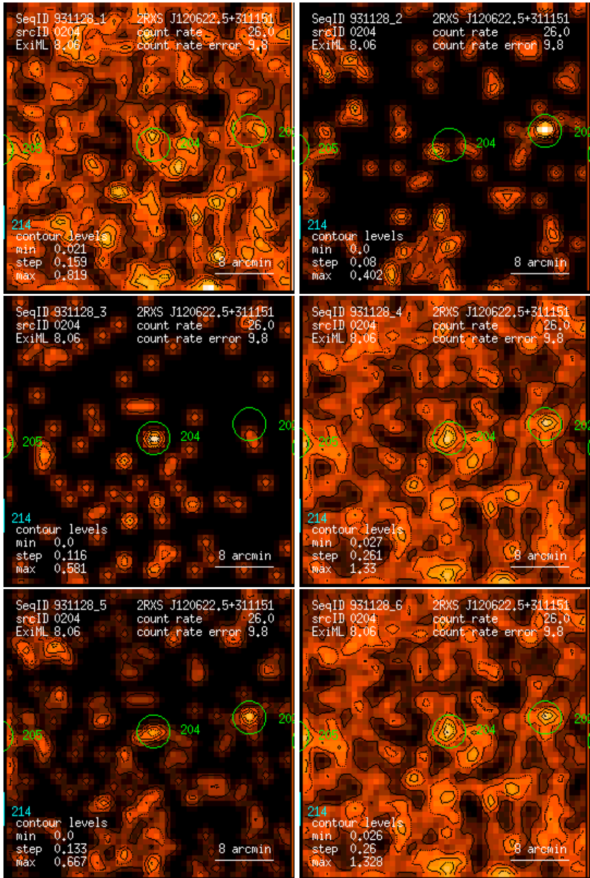
Figure 204: RASS 931128: detection 0204: band rate images, Gaussian filter: (1) PSPC channels 11 – 41, (2) 52 – 90, (3) 91 – 201, (4) 11 – 235, (5) 52 – 201, (6) 11 – 201. Broad band rates in counts/ks. Band rate contour levels in counts/ks/arcmin 2 .
