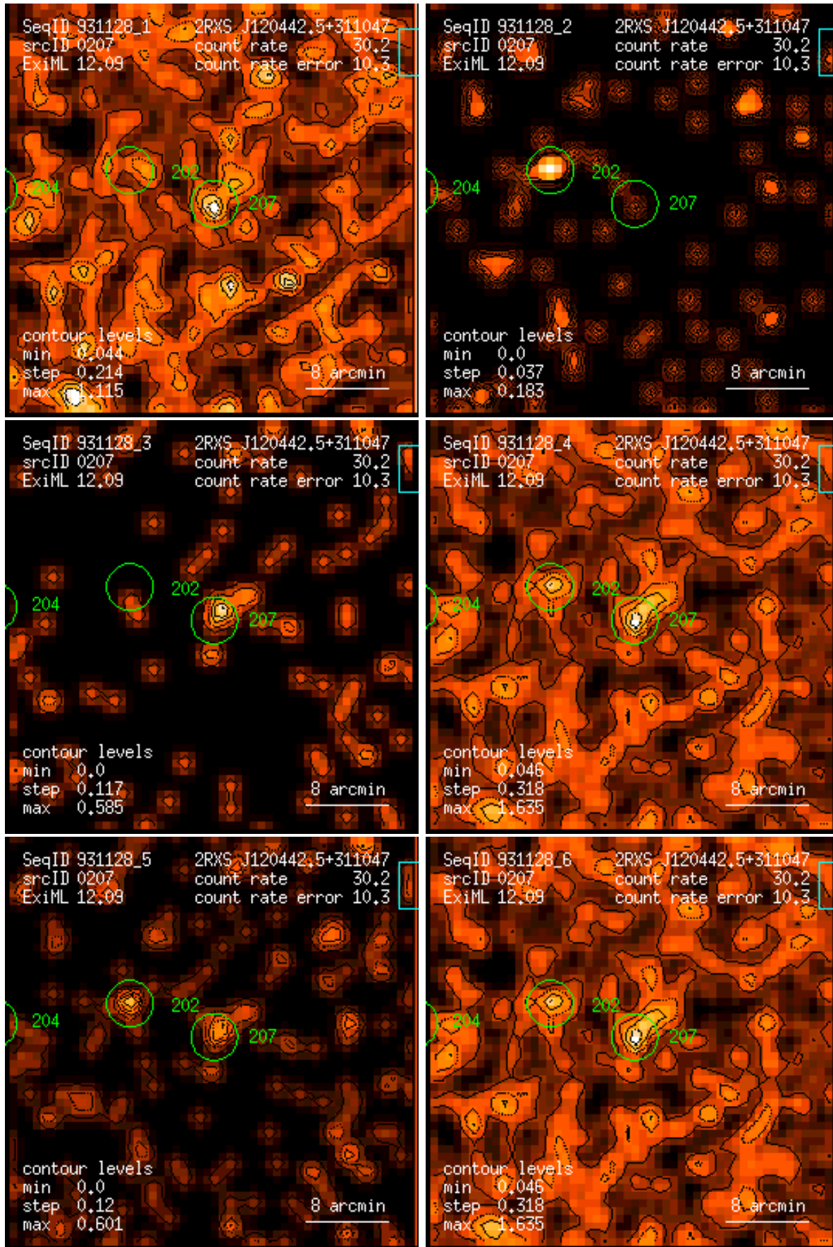
Figure 207: RASS 931128: detection 0207: band rate images, Gaussian filter: (1) PSPC channels 11 – 41, (2) 52 – 90, (3) 91 – 201, (4) 11 – 235, (5) 52 – 201, (6) 11 – 201. Broad band rates in counts/ks. Band rate contour levels in counts/ks/arcmin 2 .
