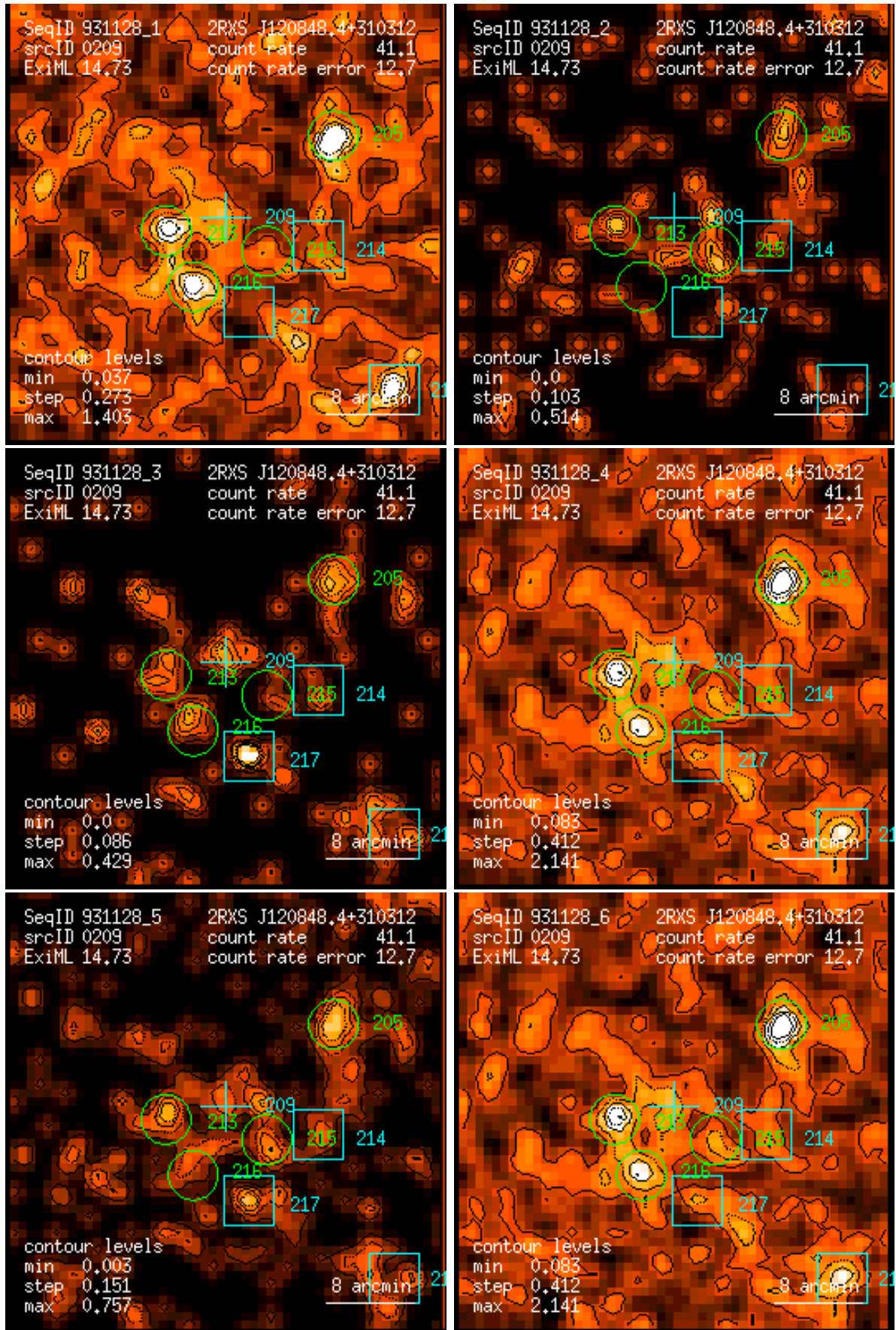
Figure 209: RASS 931128: detection 0209: band rate images, Gaussian filter: (1) PSPC channels 11 – 41, (2) 52 – 90, (3) 91 – 201, (4) 11 – 235, (5) 52 – 201, (6) 11 – 201. Broad band rates in counts/ks. Band rate contour levels in counts/ks/arcmin 2 .
