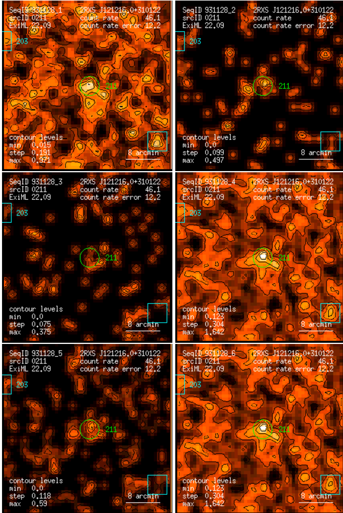
Figure 211: RASS 931128: detection 0211: band rate images, Gaussian filter: (1) PSPC channels 11 – 41, (2) 52 – 90, (3) 91 – 201, (4) 11 – 235, (5) 52 – 201, (6) 11 – 201. Broad band rates in counts/ks. Band rate contour levels in counts/ks/arcmin 2 .
