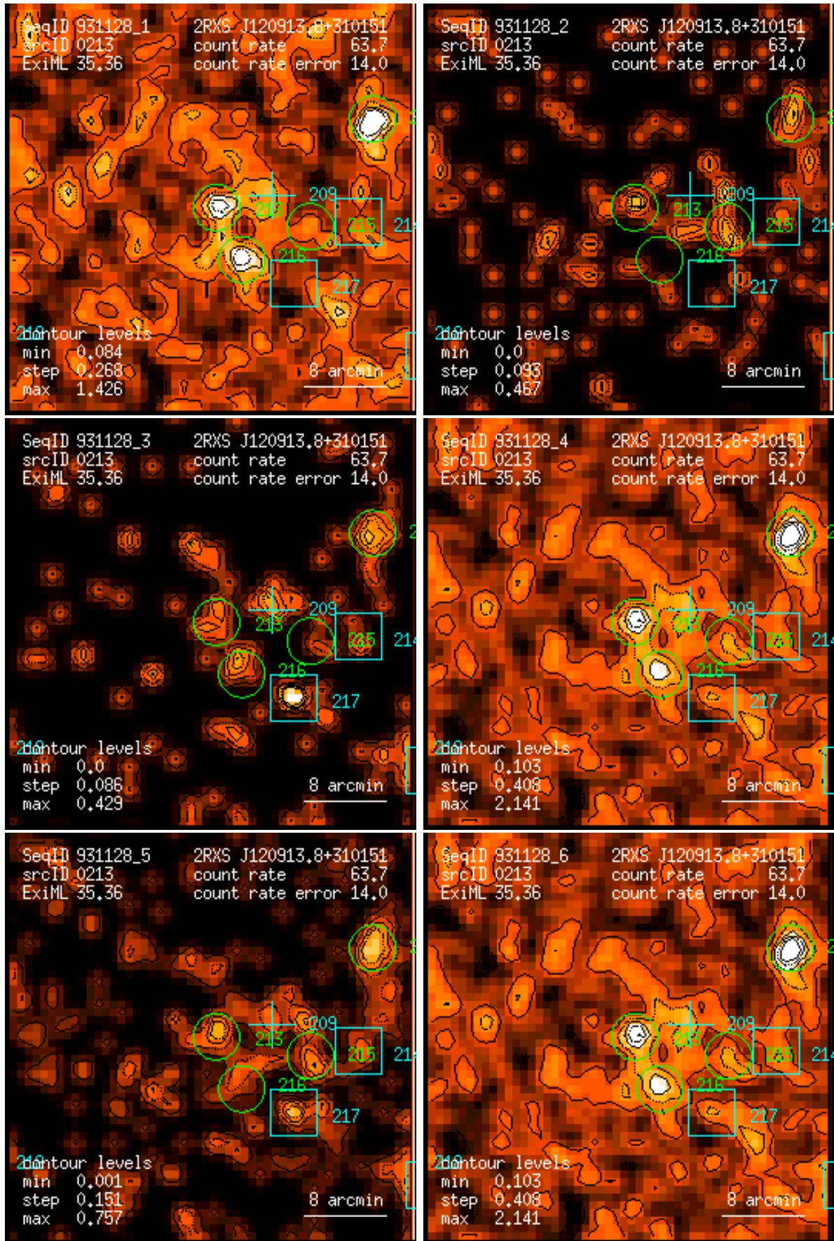
Figure 213: RASS 931128: detection 0213: band rate images, Gaussian filter: (1) PSPC channels 11 – 41, (2) 52 – 90, (3) 91 – 201, (4) 11 – 235, (5) 52 – 201, (6) 11 – 201. Broad band rates in counts/ks. Band rate contour levels in counts/ks/arcmin 2 .
