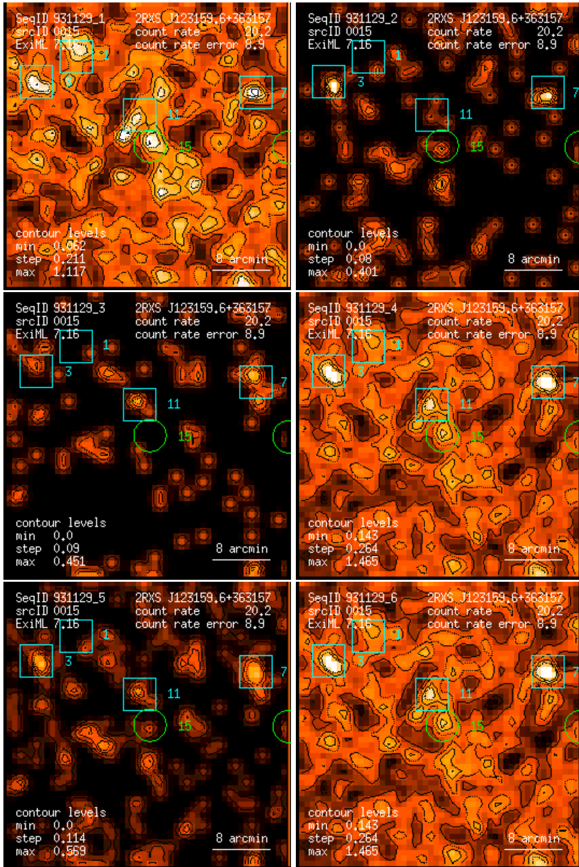
Figure 15: RASS 931129: detection 0015: band rate images, Gaussian filter: (1) PSPC channels 11 – 41, (2) 52 – 90, (3) 91 – 201, (4) 11 – 235, (5) 52 – 201, (6) 11 – 201. Broad band rates in counts/ks. Band rate contour levels in counts/ks/arcmin 2 .
