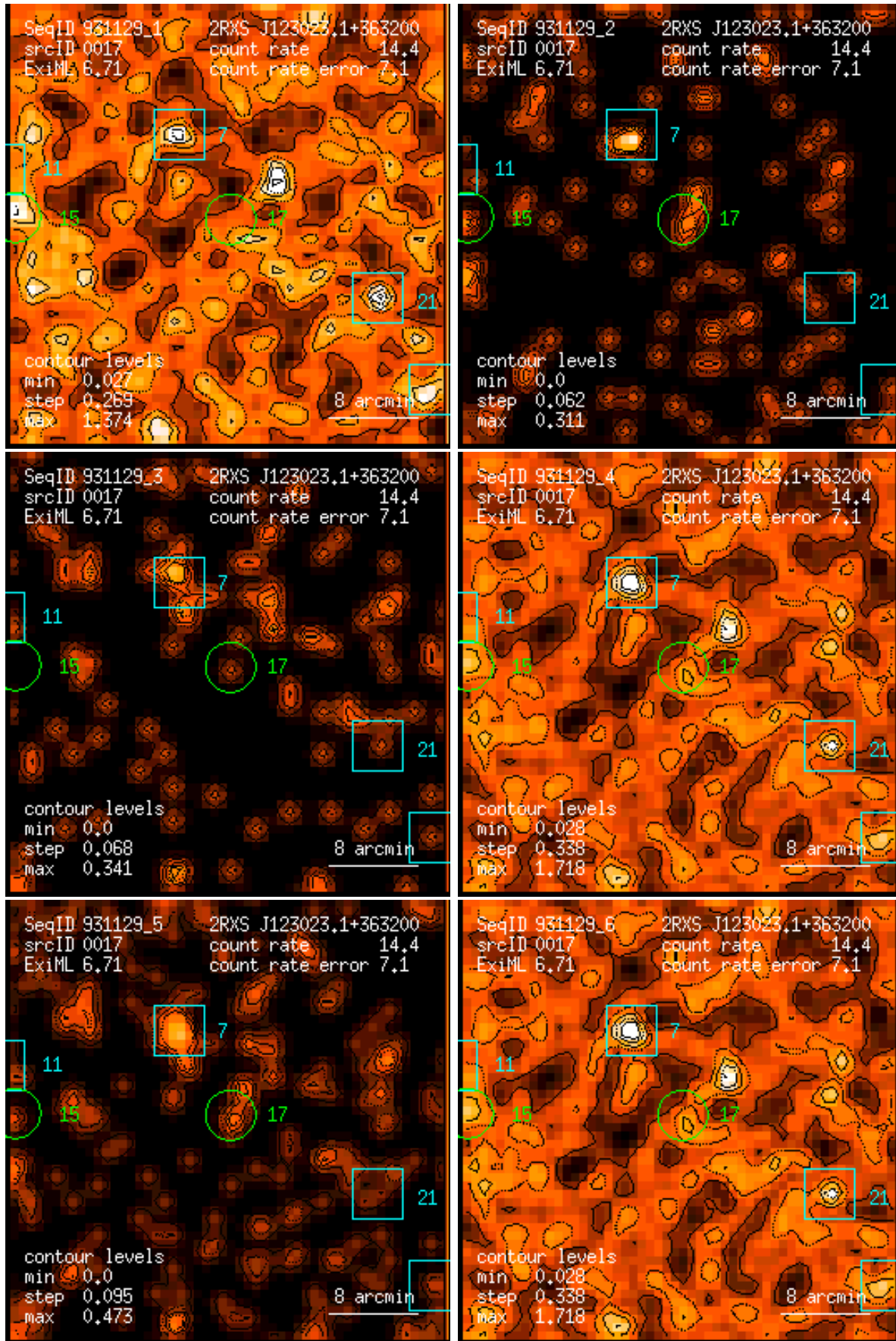
Figure 17: RASS 931129: detection 0017: band rate images, Gaussian filter: (1) PSPC channels 11 – 41, (2) 52 – 90, (3) 91 – 201, (4) 11 – 235, (5) 52 – 201, (6) 11 – 201. Broad band rates in counts/ks. Band rate contour levels in counts/ks/arcmin 2 .
