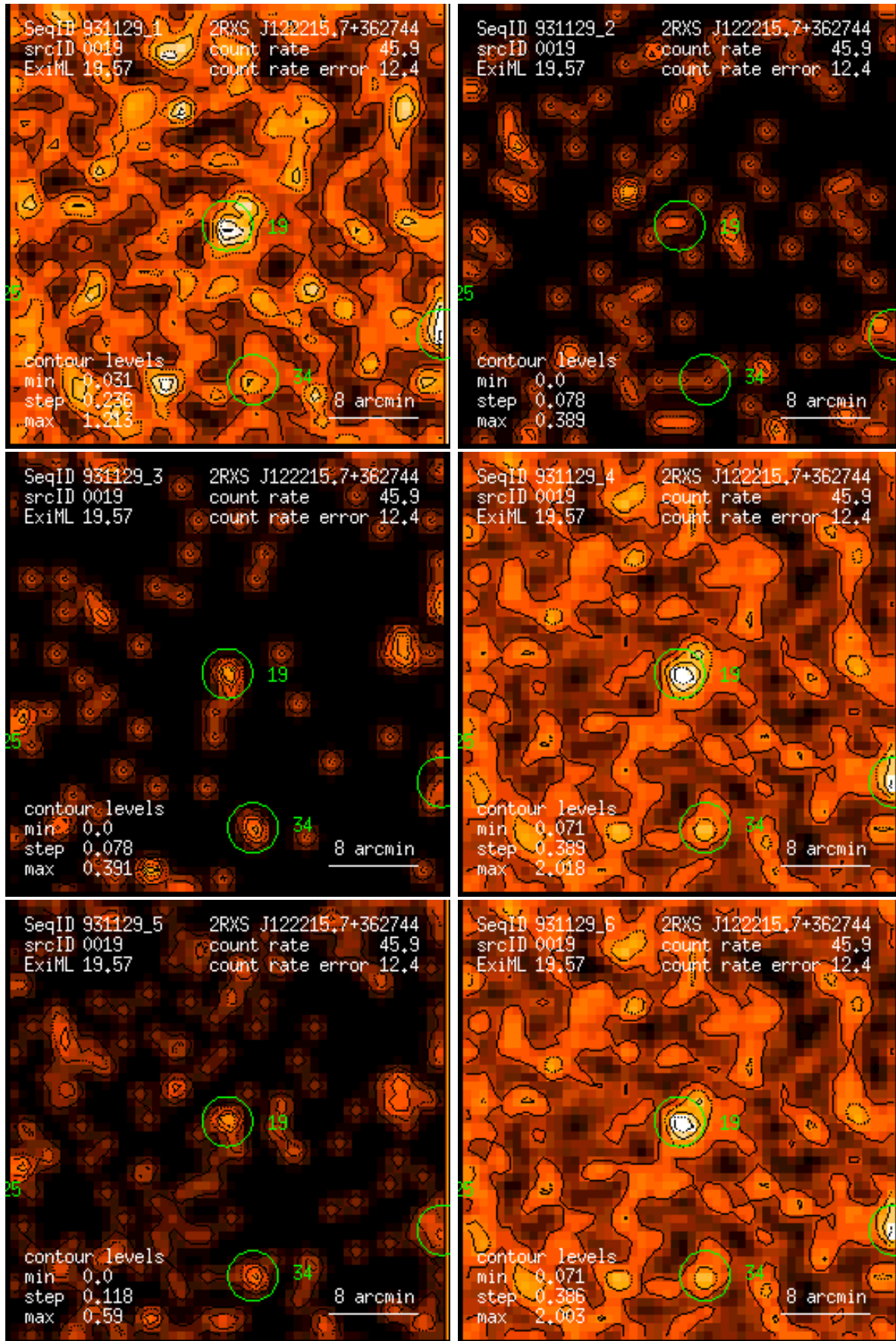
Figure 19: RASS 931129: detection 0019: band rate images, Gaussian filter: (1) PSPC channels 11 – 41, (2) 52 – 90, (3) 91 – 201, (4) 11 – 235, (5) 52 – 201, (6) 11 – 201. Broad band rates in counts/ks. Band rate contour levels in counts/ks/arcmin 2 .
