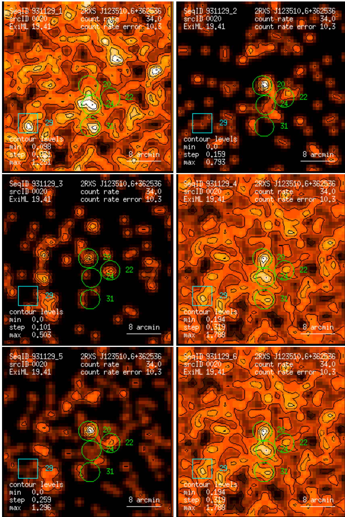
Figure 20: RASS 931129: detection 0020: band rate images, Gaussian filter: (1) PSPC channels 11 – 41, (2) 52 – 90, (3) 91 – 201, (4) 11 – 235, (5) 52 – 201, (6) 11 – 201. Broad band rates in counts/ks. Band rate contour levels in counts/ks/arcmin 2 .
