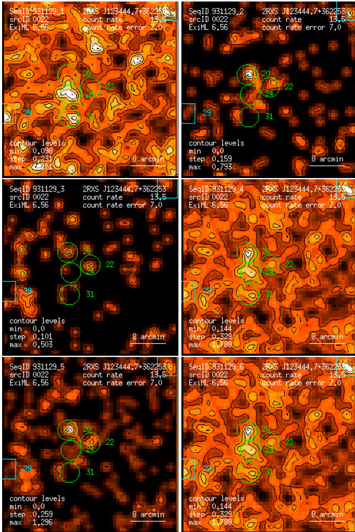
Figure 22: RASS 931129: detection 0022: band rate images, Gaussian filter: (1) PSPC channels 11 – 41, (2) 52 – 90, (3) 91 – 201, (4) 11 – 235, (5) 52 – 201, (6) 11 – 201. Broad band rates in counts/ks. Band rate contour levels in counts/ks/arcmin 2 .
