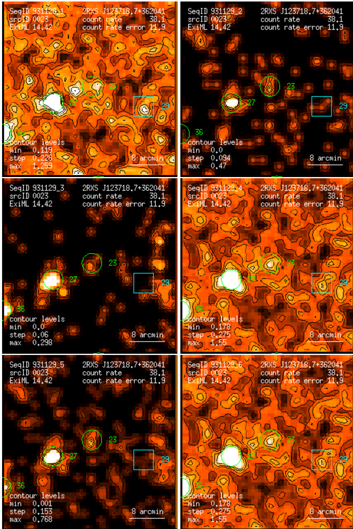
Figure 23: RASS 931129: detection 0023: band rate images, Gaussian filter: (1) PSPC channels 11 – 41, (2) 52 – 90, (3) 91 – 201, (4) 11 – 235, (5) 52 – 201, (6) 11 – 201. Broad band rates in counts/ks. Band rate contour levels in counts/ks/arcmin 2 .
