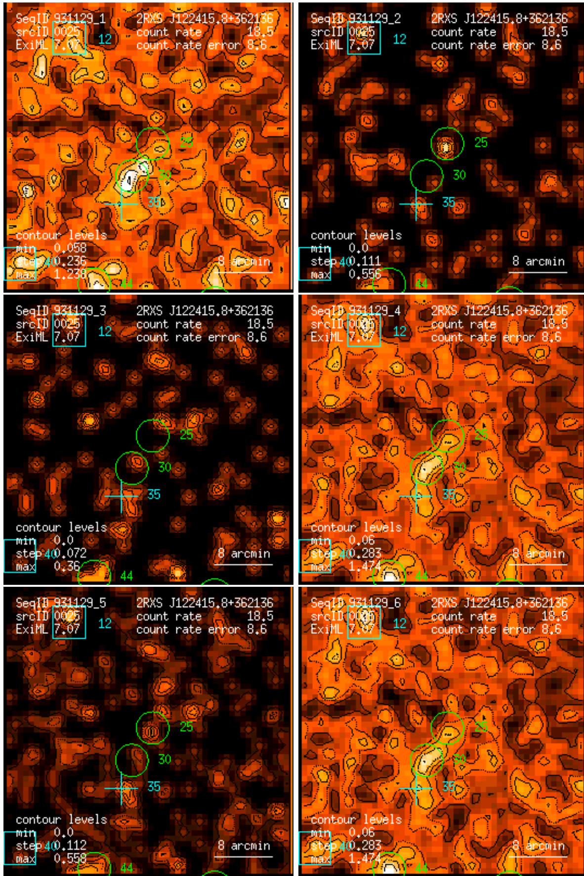
Figure 25: RASS 931129: detection 0025: band rate images, Gaussian filter: (1) PSPC channels 11 – 41, (2) 52 – 90, (3) 91 – 201, (4) 11 – 235, (5) 52 – 201, (6) 11 – 201. Broad band rates in counts/ks. Band rate contour levels in counts/ks/arcmin 2 .
