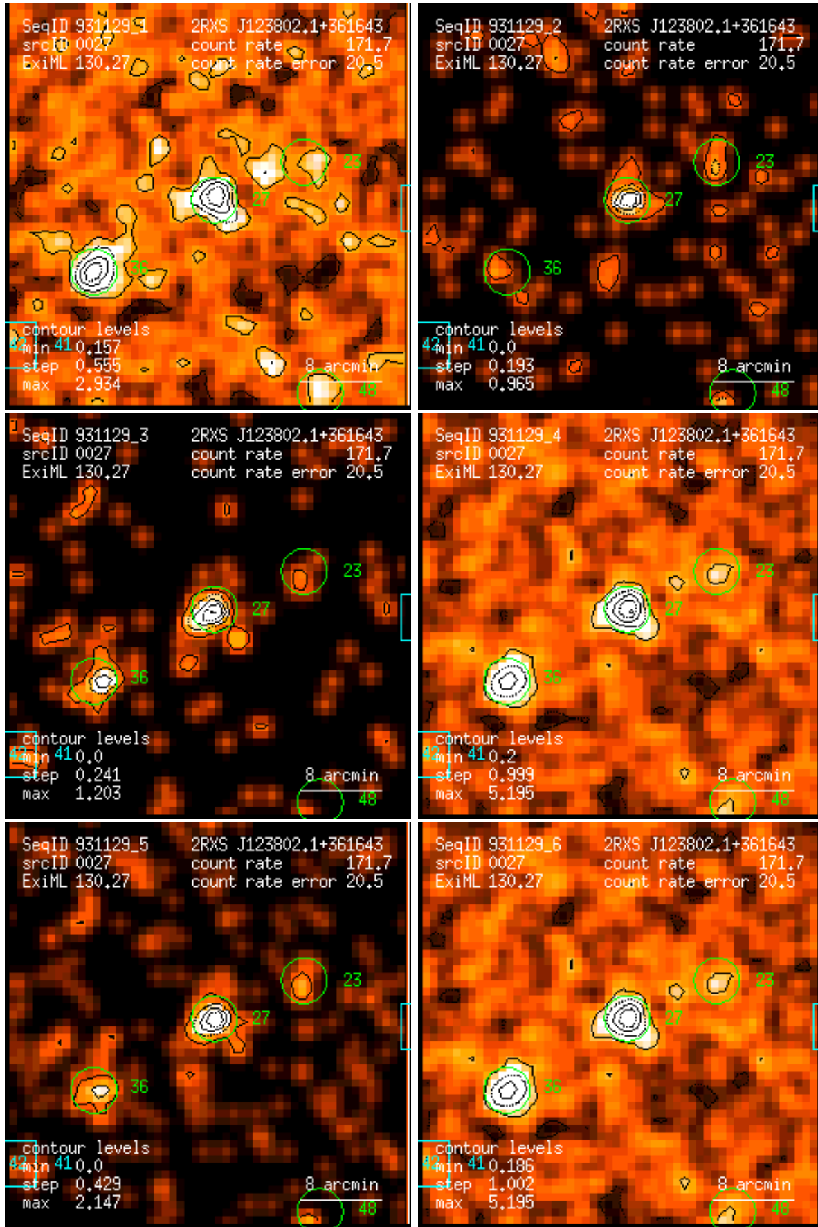
Figure 27: RASS 931129: detection 0027: band rate images, Gaussian filter: (1) PSPC channels 11 – 41, (2) 52 – 90, (3) 91 – 201, (4) 11 – 235, (5) 52 – 201, (6) 11 – 201. Broad band rates in counts/ks. Band rate contour levels in counts/ks/arcmin 2 .
