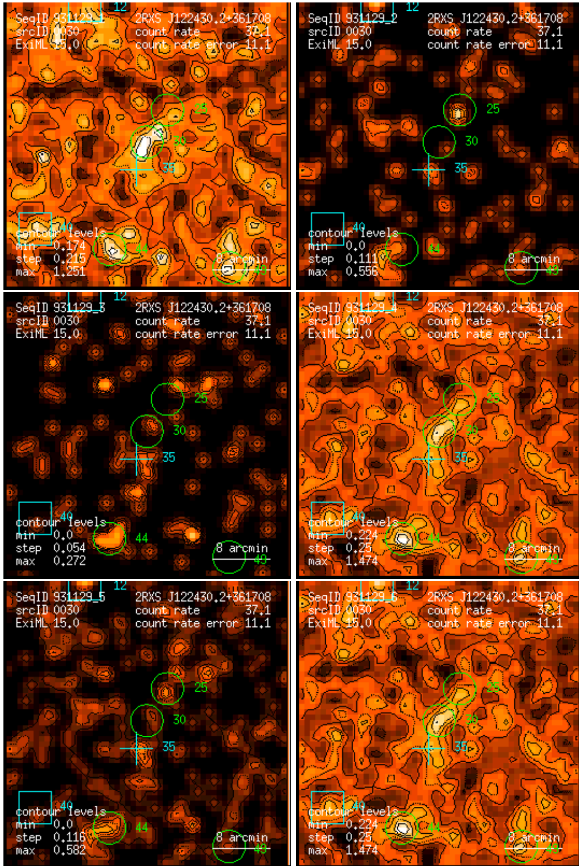
Figure 30: RASS 931129: detection 0030: band rate images, Gaussian filter: (1) PSPC channels 11 – 41, (2) 52 – 90, (3) 91 – 201, (4) 11 – 235, (5) 52 – 201, (6) 11 – 201. Broad band rates in counts/ks. Band rate contour levels in counts/ks/arcmin 2 .
