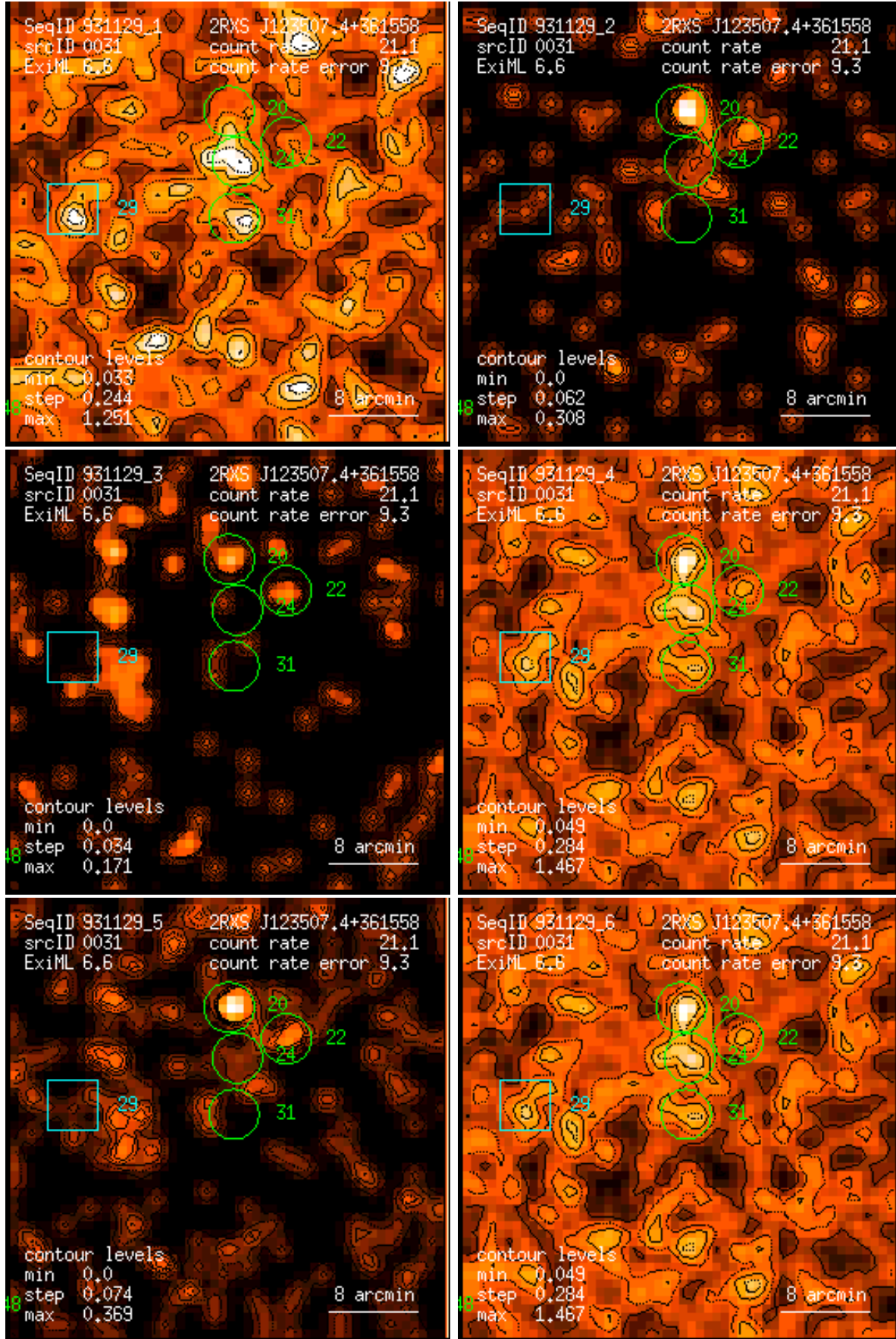
Figure 31: RASS 931129: detection 0031: band rate images, Gaussian filter: (1) PSPC channels 11 – 41, (2) 52 – 90, (3) 91 – 201, (4) 11 – 235, (5) 52 – 201, (6) 11 – 201. Broad band rates in counts/ks. Band rate contour levels in counts/ks/arcmin 2 .
