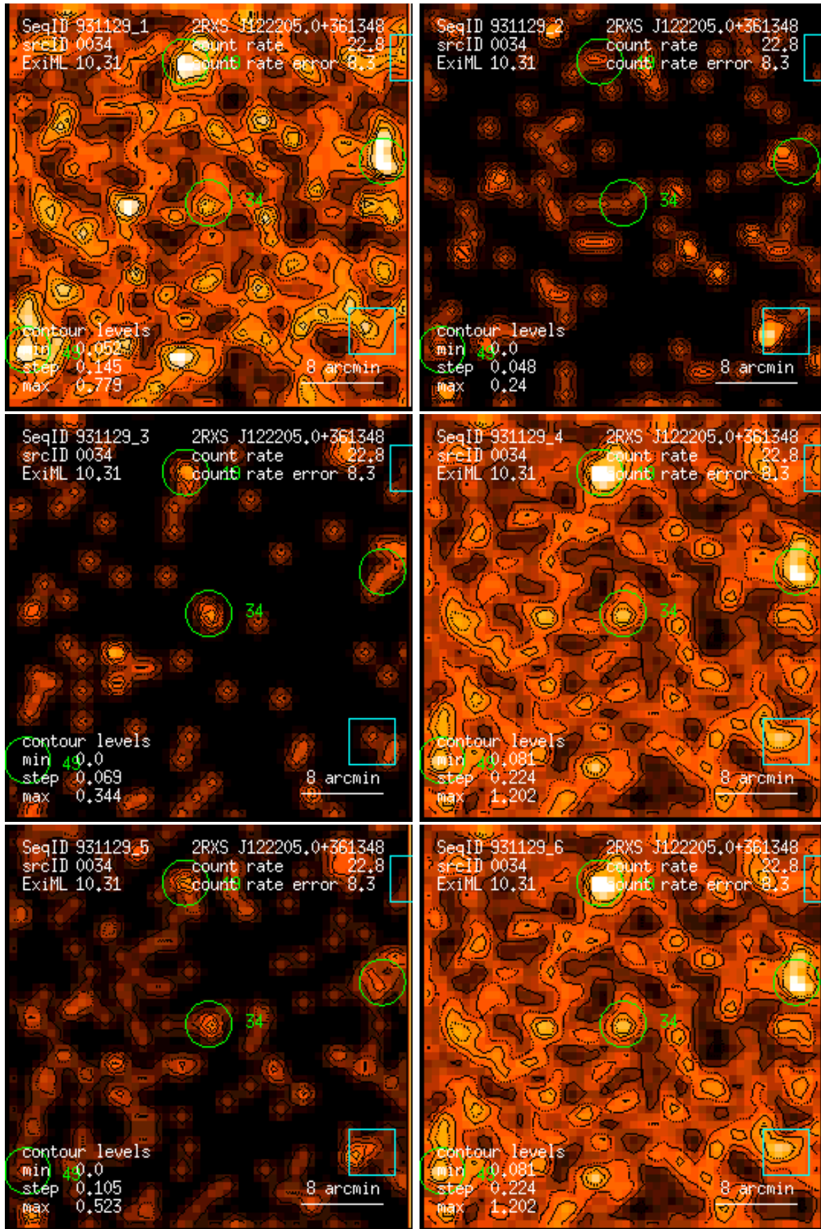
Figure 34: RASS 931129: detection 0034: band rate images, Gaussian filter: (1) PSPC channels 11 – 41, (2) 52 – 90, (3) 91 – 201, (4) 11 – 235, (5) 52 – 201, (6) 11 – 201. Broad band rates in counts/ks. Band rate contour levels in counts/ks/arcmin 2 .
