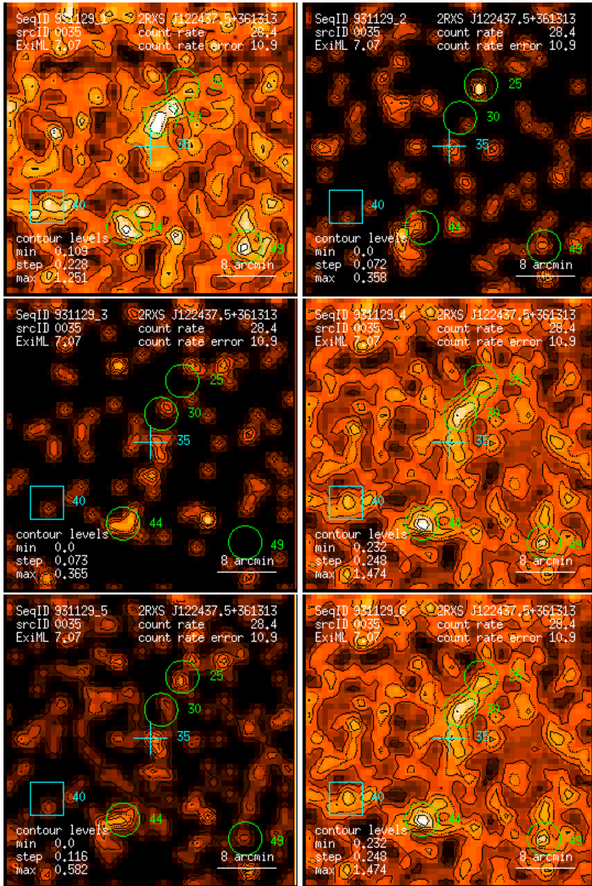
Figure 35: RASS 931129: detection 0035: band rate images, Gaussian filter: (1) PSPC channels 11 – 41, (2) 52 – 90, (3) 91 – 201, (4) 11 – 235, (5) 52 – 201, (6) 11 – 201. Broad band rates in counts/ks. Band rate contour levels in counts/ks/arcmin 2 .
