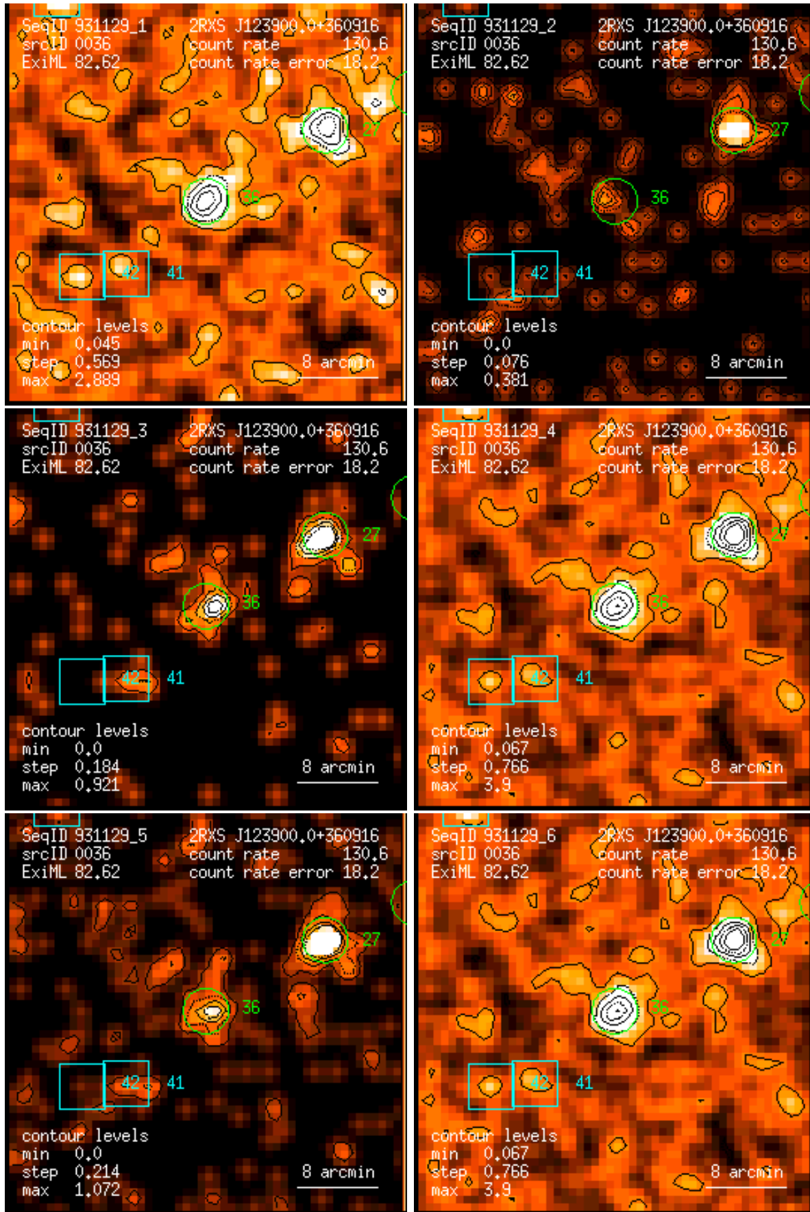
Figure 36: RASS 931129: detection 0036: band rate images, Gaussian filter: (1) PSPC channels 11 – 41, (2) 52 – 90, (3) 91 – 201, (4) 11 – 235, (5) 52 – 201, (6) 11 – 201. Broad band rates in counts/ks. Band rate contour levels in counts/ks/arcmin 2 .
