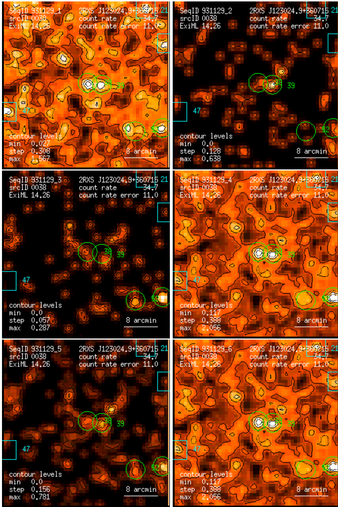
Figure 38: RASS 931129: detection 0038: band rate images, Gaussian filter: (1) PSPC channels 11 – 41, (2) 52 – 90, (3) 91 – 201, (4) 11 – 235, (5) 52 – 201, (6) 11 – 201. Broad band rates in counts/ks. Band rate contour levels in counts/ks/arcmin 2 .
