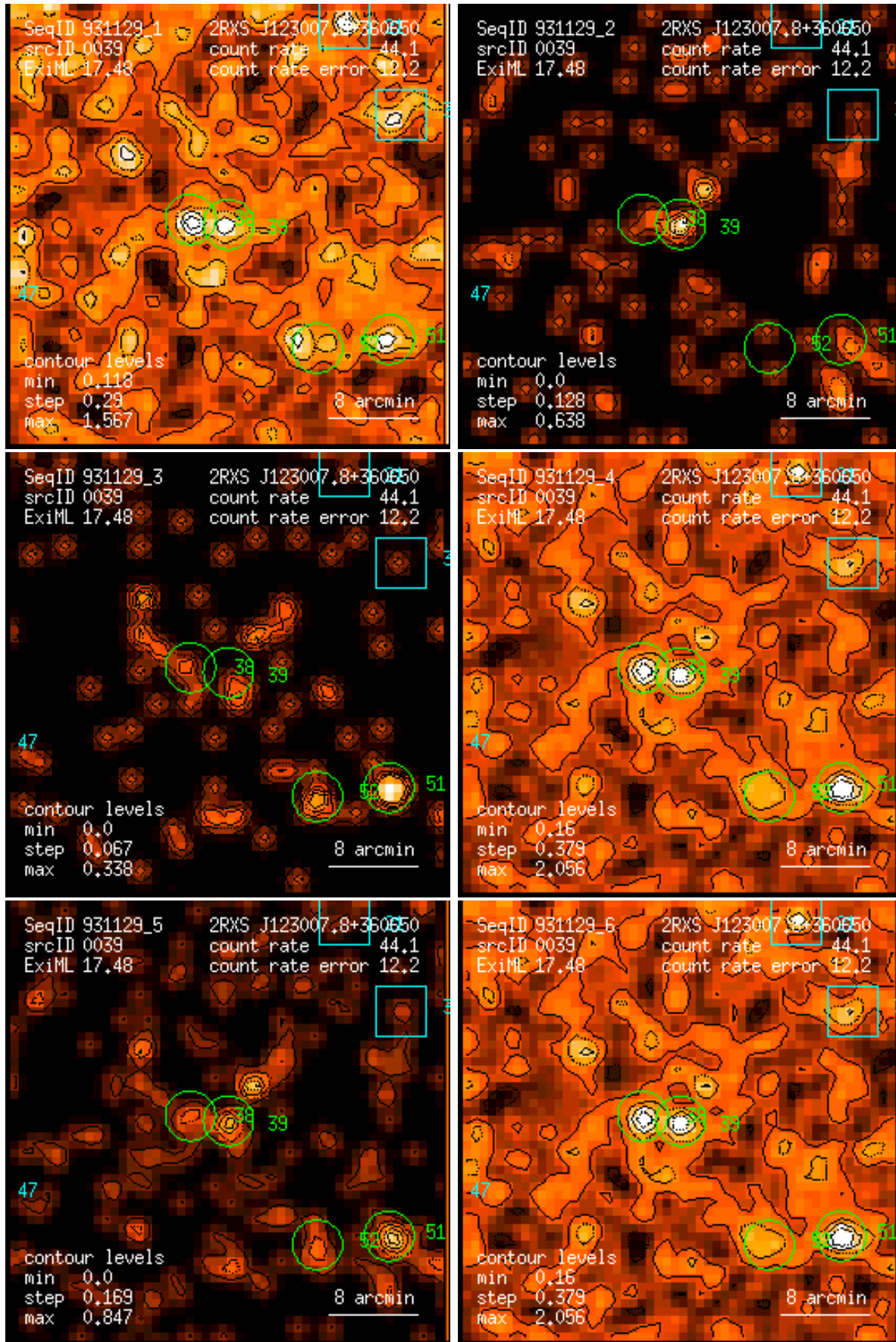
Figure 39: RASS 931129: detection 0039: band rate images, Gaussian filter: (1) PSPC channels 11 – 41, (2) 52 – 90, (3) 91 – 201, (4) 11 – 235, (5) 52 – 201, (6) 11 – 201. Broad band rates in counts/ks. Band rate contour levels in counts/ks/arcmin 2 .
