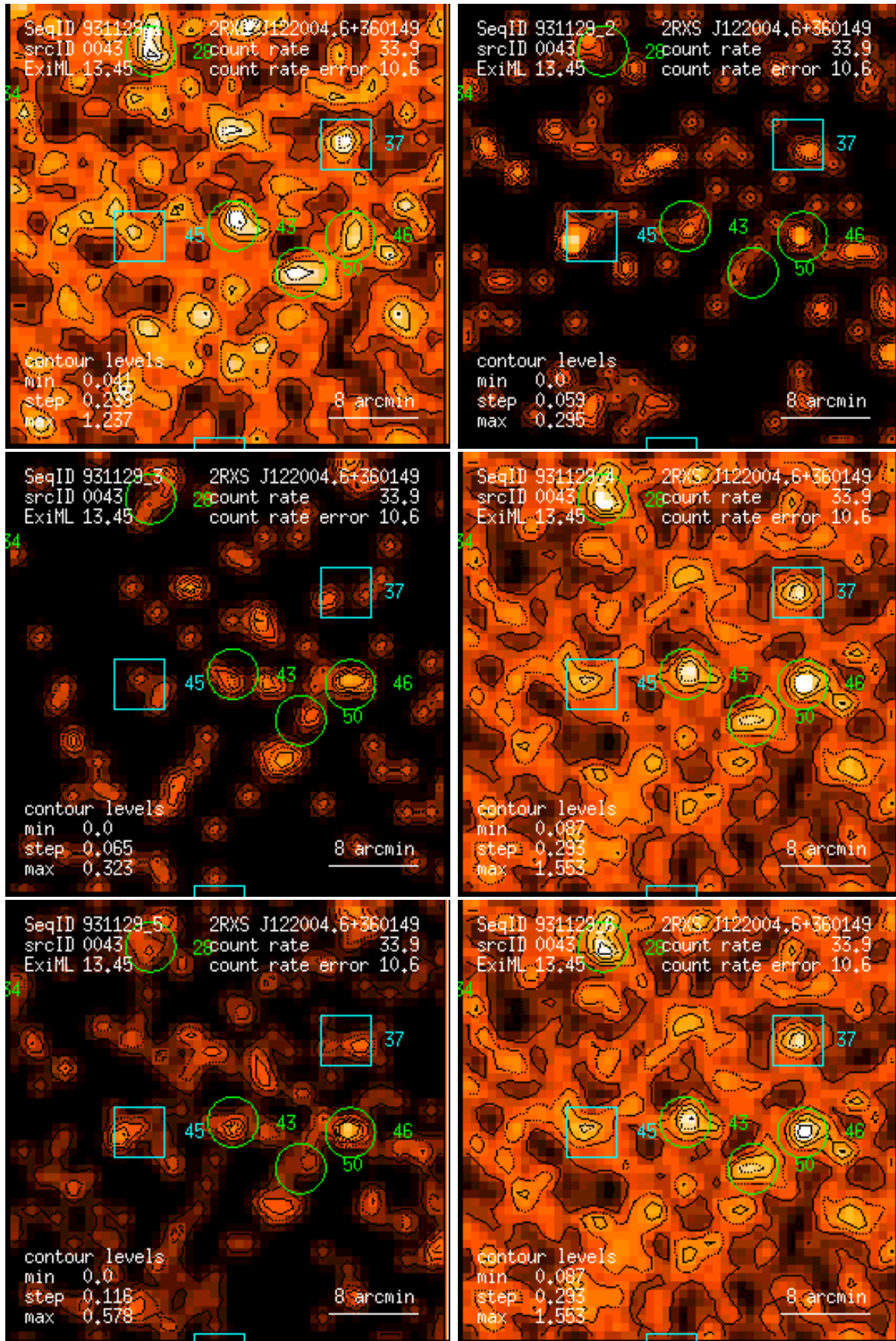
Figure 43: RASS 931129: detection 0043: band rate images, Gaussian filter: (1) PSPC channels 11 – 41, (2) 52 – 90, (3) 91 – 201, (4) 11 – 235, (5) 52 – 201, (6) 11 – 201. Broad band rates in counts/ks. Band rate contour levels in counts/ks/arcmin 2 .
