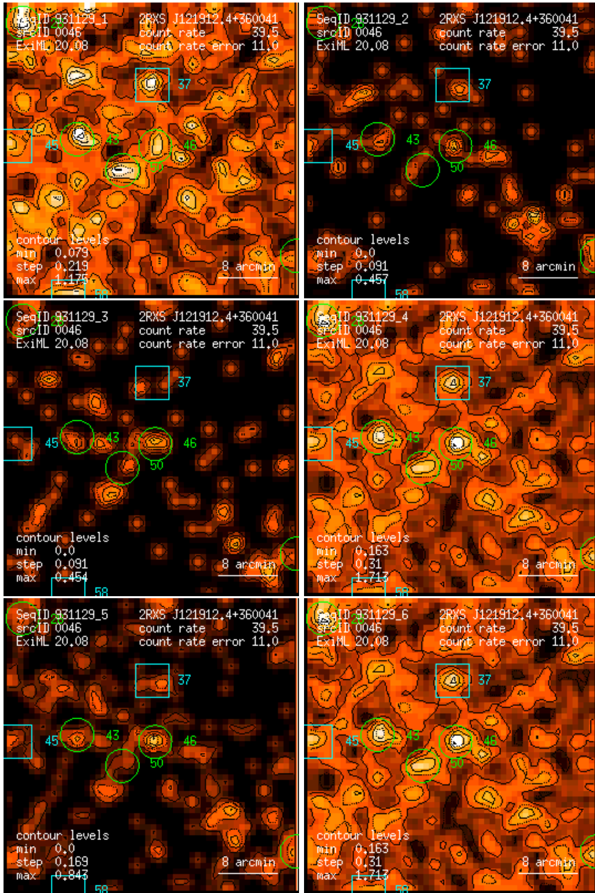
Figure 46: RASS 931129: detection 0046: band rate images, Gaussian filter: (1) PSPC channels 11 – 41, (2) 52 – 90, (3) 91 – 201, (4) 11 – 235, (5) 52 – 201, (6) 11 – 201. Broad band rates in counts/ks. Band rate contour levels in counts/ks/arcmin 2 .
