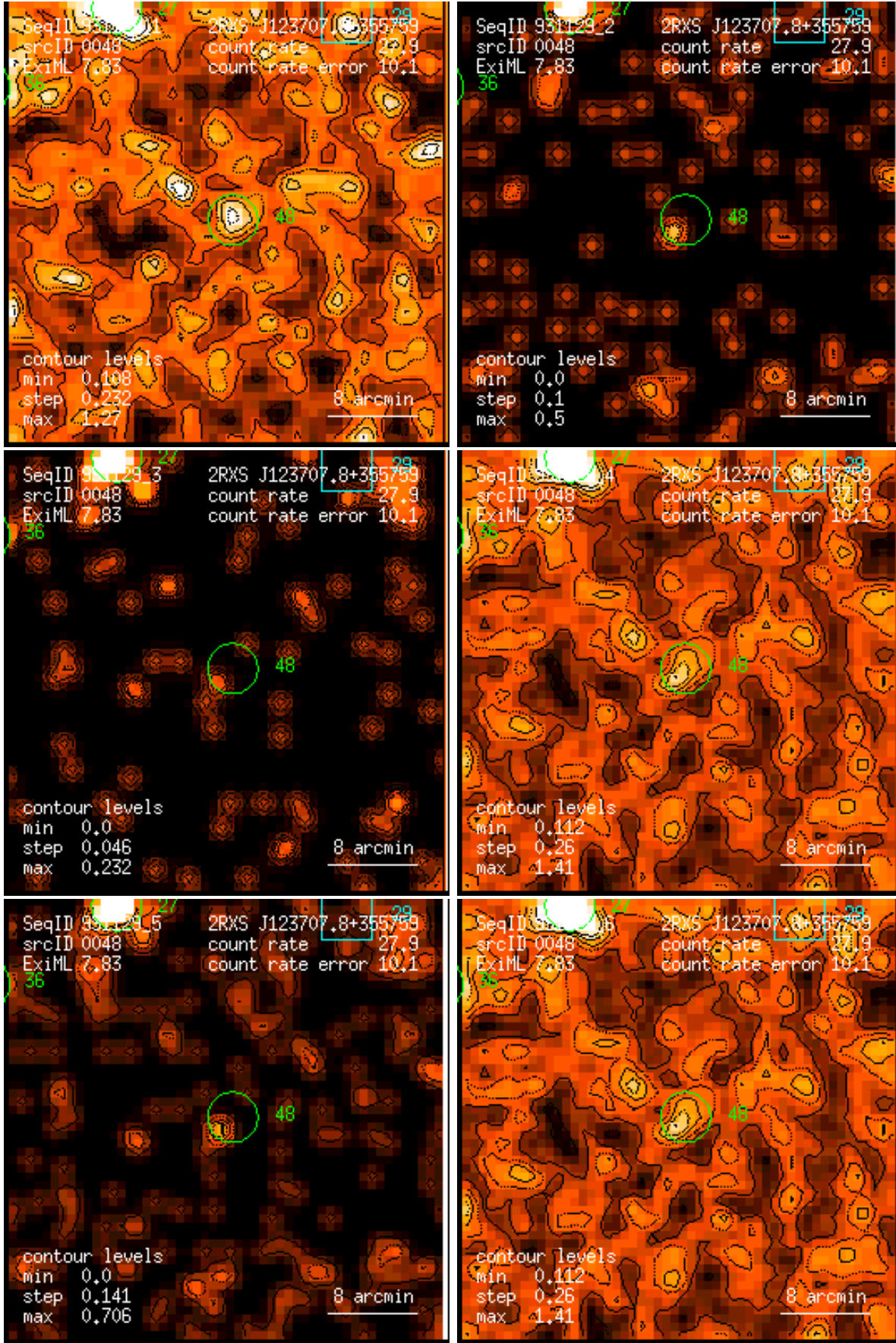
Figure 48: RASS 931129: detection 0048: band rate images, Gaussian filter: (1) PSPC channels 11 – 41, (2) 52 – 90, (3) 91 – 201, (4) 11 – 235, (5) 52 – 201, (6) 11 – 201. Broad band rates in counts/ks. Band rate contour levels in counts/ks/arcmin 2 .
