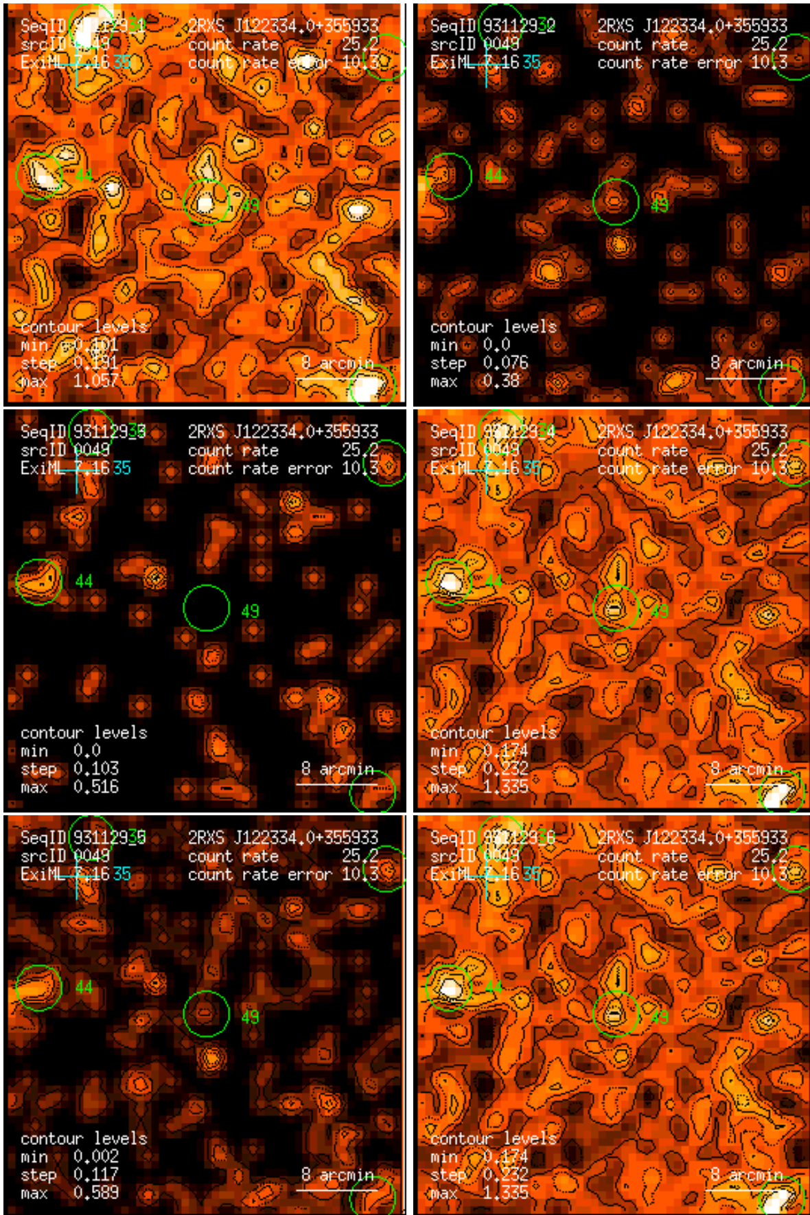
Figure 49: RASS 931129: detection 0049: band rate images, Gaussian filter: (1) PSPC channels 11 – 41, (2) 52 – 90, (3) 91 – 201, (4) 11 – 235, (5) 52 – 201, (6) 11 – 201. Broad band rates in counts/ks. Band rate contour levels in counts/ks/arcmin 2 .
