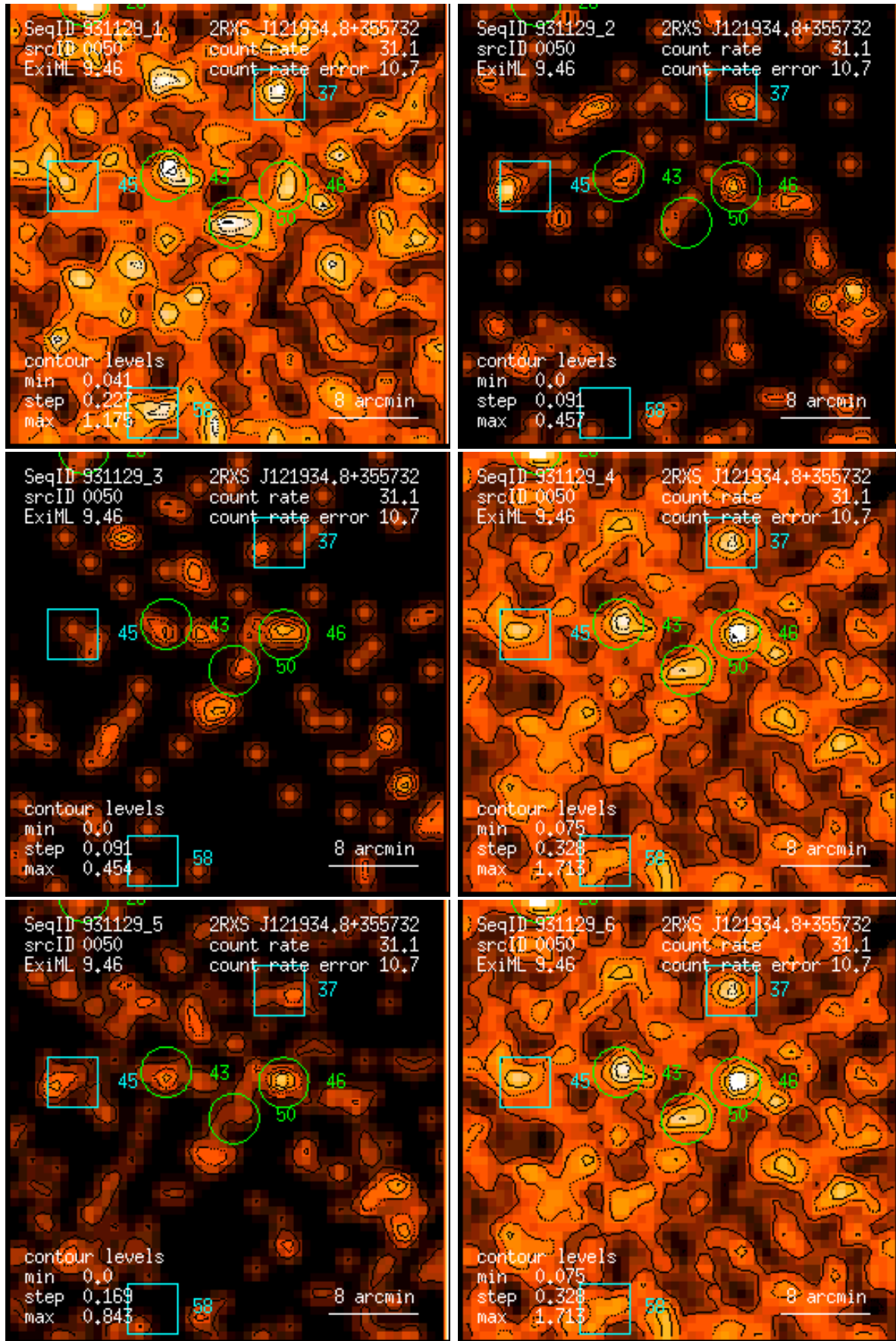
Figure 50: RASS 931129: detection 0050: band rate images, Gaussian filter: (1) PSPC channels 11 – 41, (2) 52 – 90, (3) 91 – 201, (4) 11 – 235, (5) 52 – 201, (6) 11 – 201. Broad band rates in counts/ks. Band rate contour levels in counts/ks/arcmin 2 .
