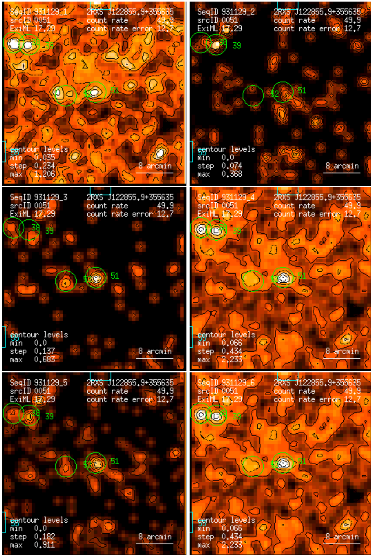
Figure 51: RASS 931129: detection 0051: band rate images, Gaussian filter: (1) PSPC channels 11 – 41, (2) 52 – 90, (3) 91 – 201, (4) 11 – 235, (5) 52 – 201, (6) 11 – 201. Broad band rates in counts/ks. Band rate contour levels in counts/ks/arcmin 2 .
