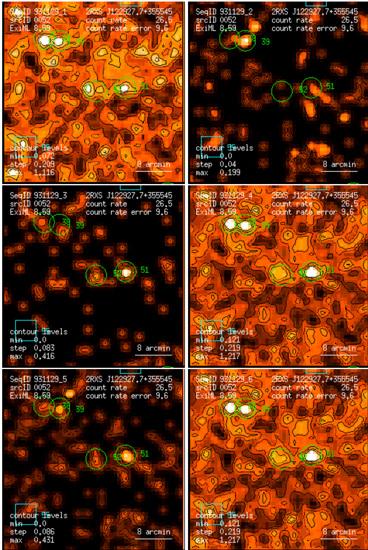
Figure 52: RASS 931129: detection 0052: band rate images, Gaussian filter: (1) PSPC channels 11 – 41, (2) 52 – 90, (3) 91 – 201, (4) 11 – 235, (5) 52 – 201, (6) 11 – 201. Broad band rates in counts/ks. Band rate contour levels in counts/ks/arcmin 2 .
