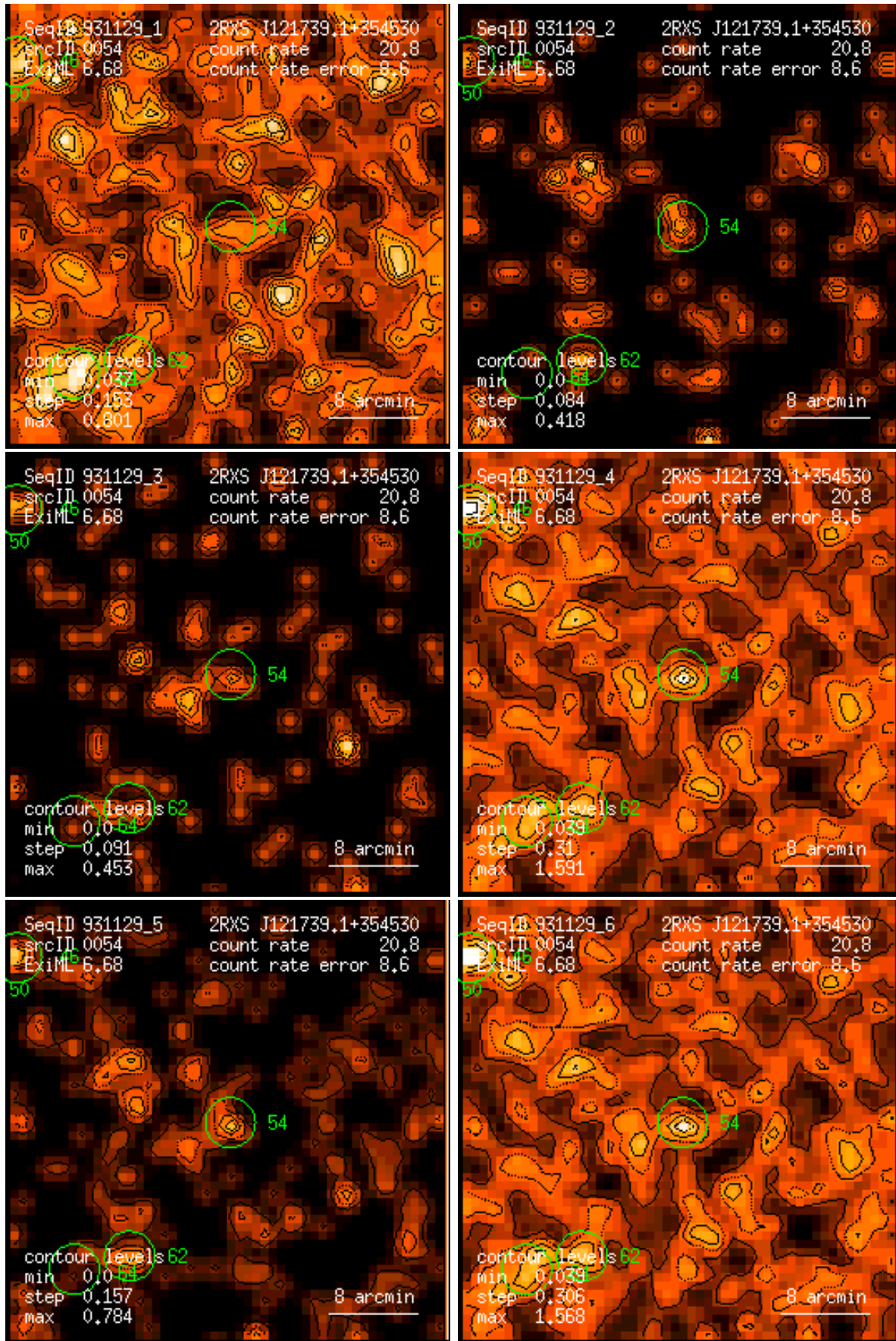
Figure 54: RASS 931129: detection 0054: band rate images, Gaussian filter: (1) PSPC channels 11 – 41, (2) 52 – 90, (3) 91 – 201, (4) 11 – 235, (5) 52 – 201, (6) 11 – 201. Broad band rates in counts/ks. Band rate contour levels in counts/ks/arcmin 2 .
