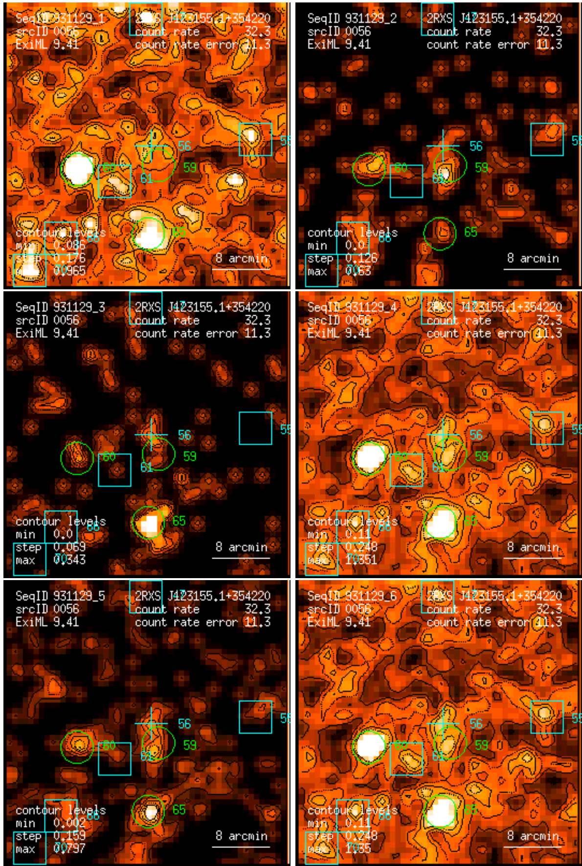
Figure 56: RASS 931129: detection 0056: band rate images, Gaussian filter: (1) PSPC channels 11 – 41, (2) 52 – 90, (3) 91 – 201, (4) 11 – 235, (5) 52 – 201, (6) 11 – 201. Broad band rates in counts/ks. Band rate contour levels in counts/ks/arcmin 2 .
