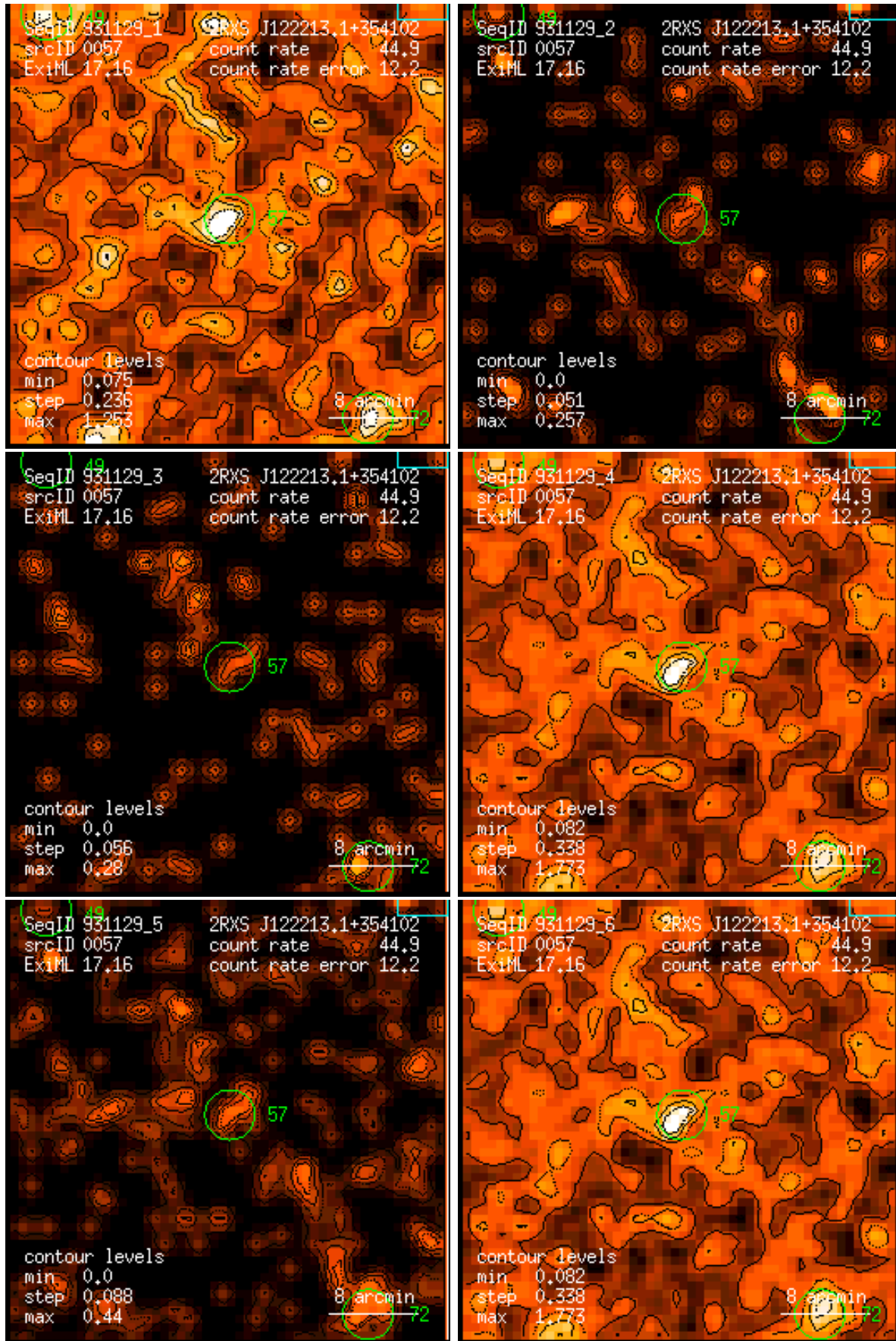
Figure 57: RASS 931129: detection 0057: band rate images, Gaussian filter: (1) PSPC channels 11 – 41, (2) 52 – 90, (3) 91 – 201, (4) 11 – 235, (5) 52 – 201, (6) 11 – 201. Broad band rates in counts/ks. Band rate contour levels in counts/ks/arcmin 2 .
