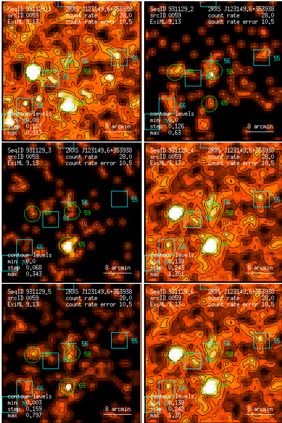
Figure 59: RASS 931129: detection 0059: band rate images, Gaussian filter: (1) PSPC channels 11 – 41, (2) 52 – 90, (3) 91 – 201, (4) 11 – 235, (5) 52 – 201, (6) 11 – 201. Broad band rates in counts/ks. Band rate contour levels in counts/ks/arcmin 2 .
