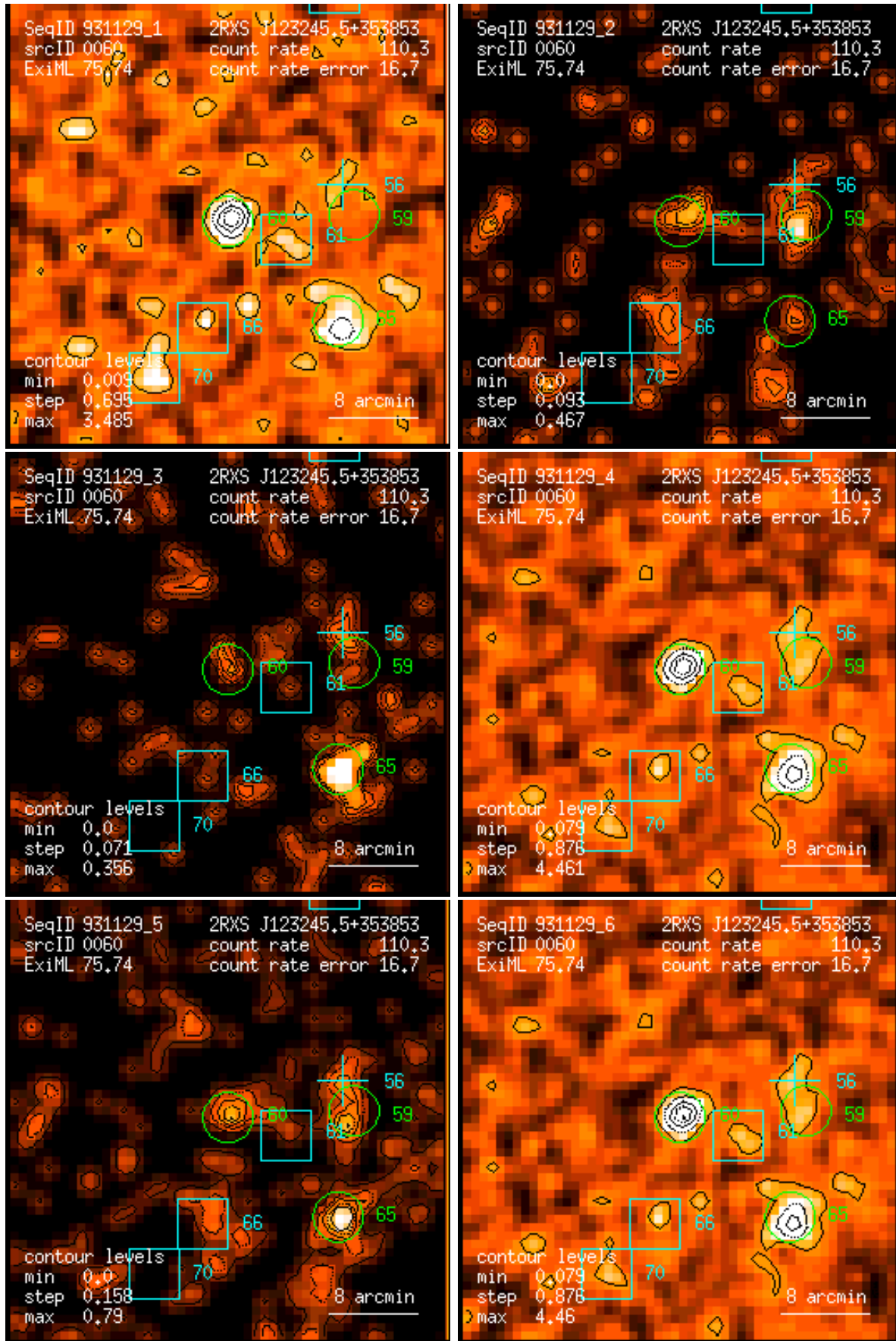
Figure 60: RASS 931129: detection 0060: band rate images, Gaussian filter: (1) PSPC channels 11 – 41, (2) 52 – 90, (3) 91 – 201, (4) 11 – 235, (5) 52 – 201, (6) 11 – 201. Broad band rates in counts/ks. Band rate contour levels in counts/ks/arcmin 2 .
