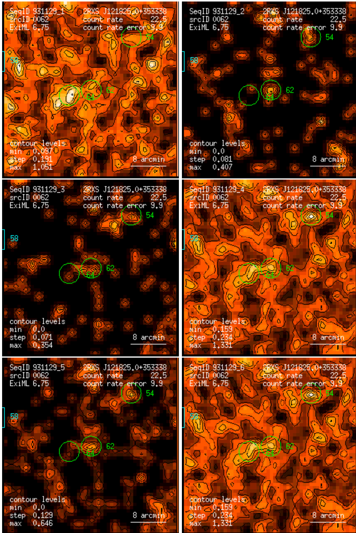
Figure 62: RASS 931129: detection 0062: band rate images, Gaussian filter: (1) PSPC channels 11 – 41, (2) 52 – 90, (3) 91 – 201, (4) 11 – 235, (5) 52 – 201, (6) 11 – 201. Broad band rates in counts/ks. Band rate contour levels in counts/ks/arcmin 2 .
