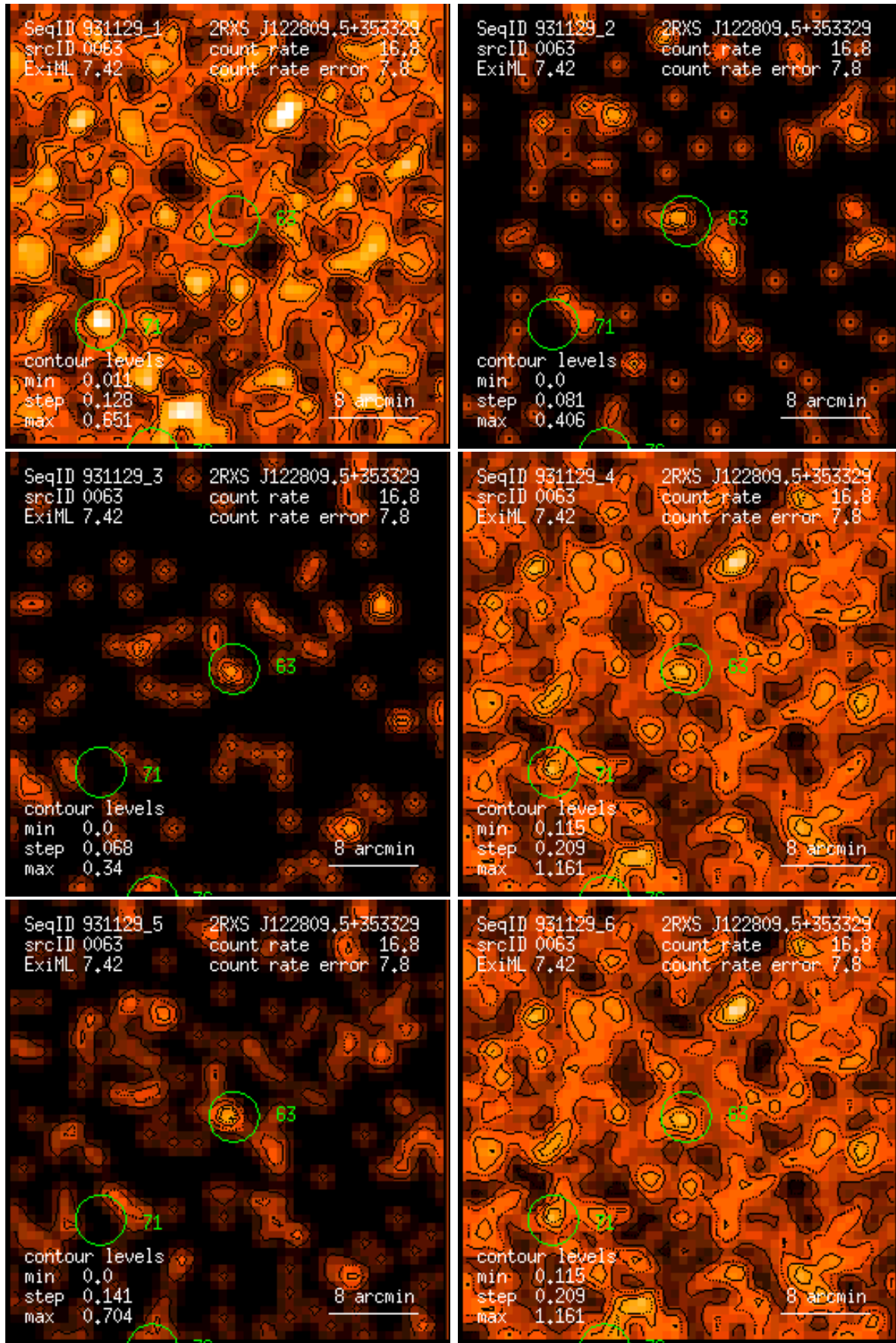
Figure 63: RASS 931129: detection 0063: band rate images, Gaussian filter: (1) PSPC channels 11 – 41, (2) 52 – 90, (3) 91 – 201, (4) 11 – 235, (5) 52 – 201, (6) 11 – 201. Broad band rates in counts/ks. Band rate contour levels in counts/ks/arcmin 2 .
