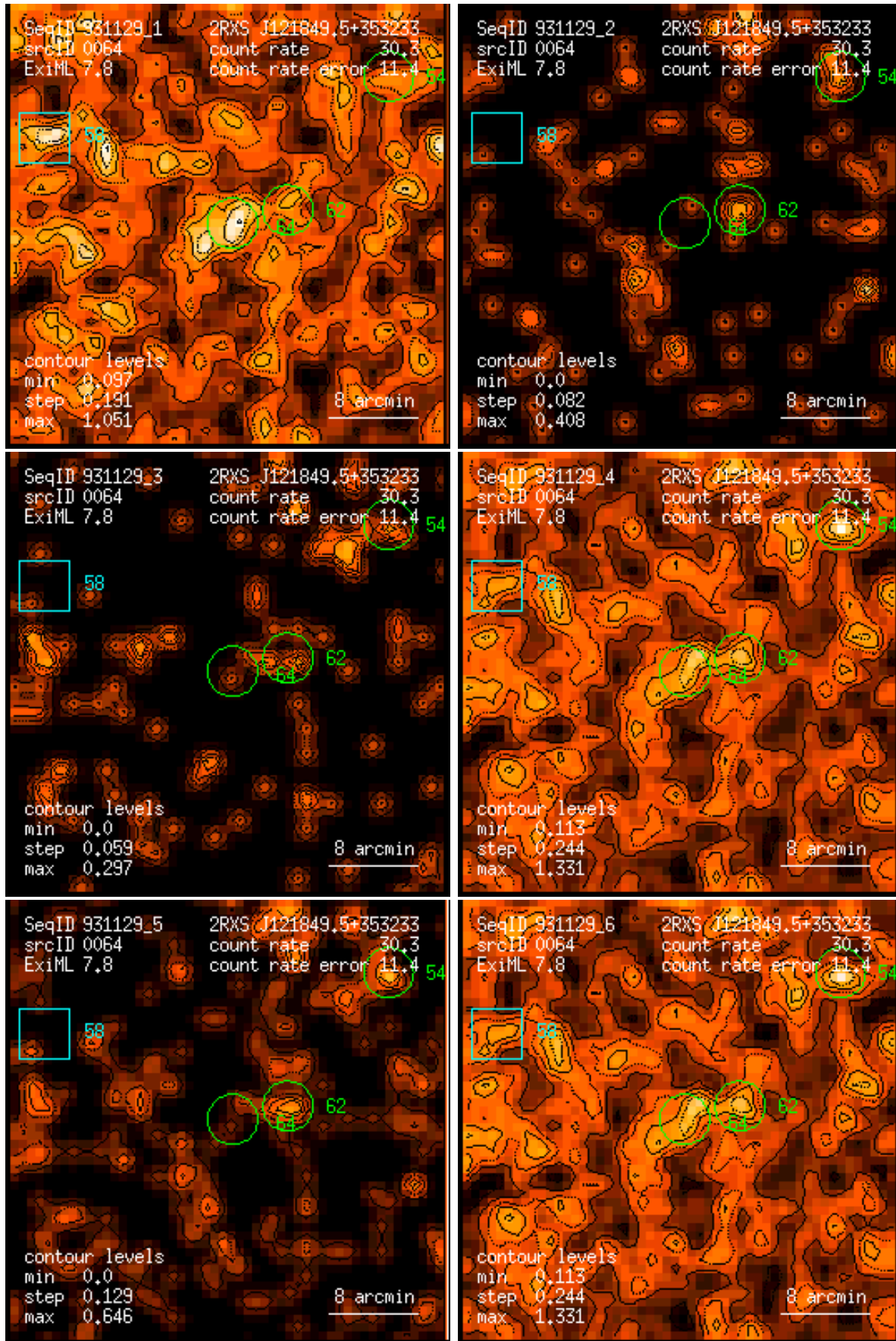
Figure 64: RASS 931129: detection 0064: band rate images, Gaussian filter: (1) PSPC channels 11 – 41, (2) 52 – 90, (3) 91 – 201, (4) 11 – 235, (5) 52 – 201, (6) 11 – 201. Broad band rates in counts/ks. Band rate contour levels in counts/ks/arcmin 2 .
