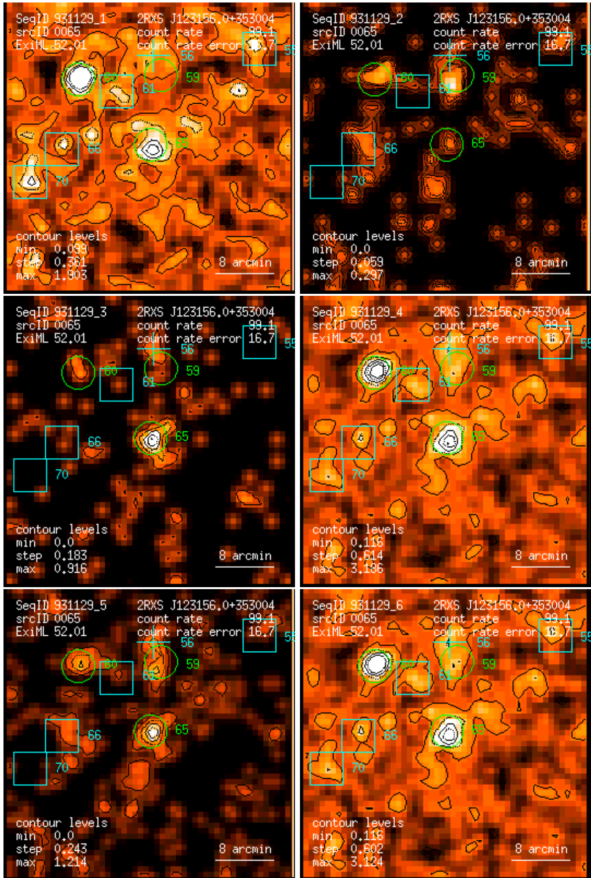
Figure 65: RASS 931129: detection 0065: band rate images, Gaussian filter: (1) PSPC channels 11 – 41, (2) 52 – 90, (3) 91 – 201, (4) 11 – 235, (5) 52 – 201, (6) 11 – 201. Broad band rates in counts/ks. Band rate contour levels in counts/ks/arcmin 2 .
