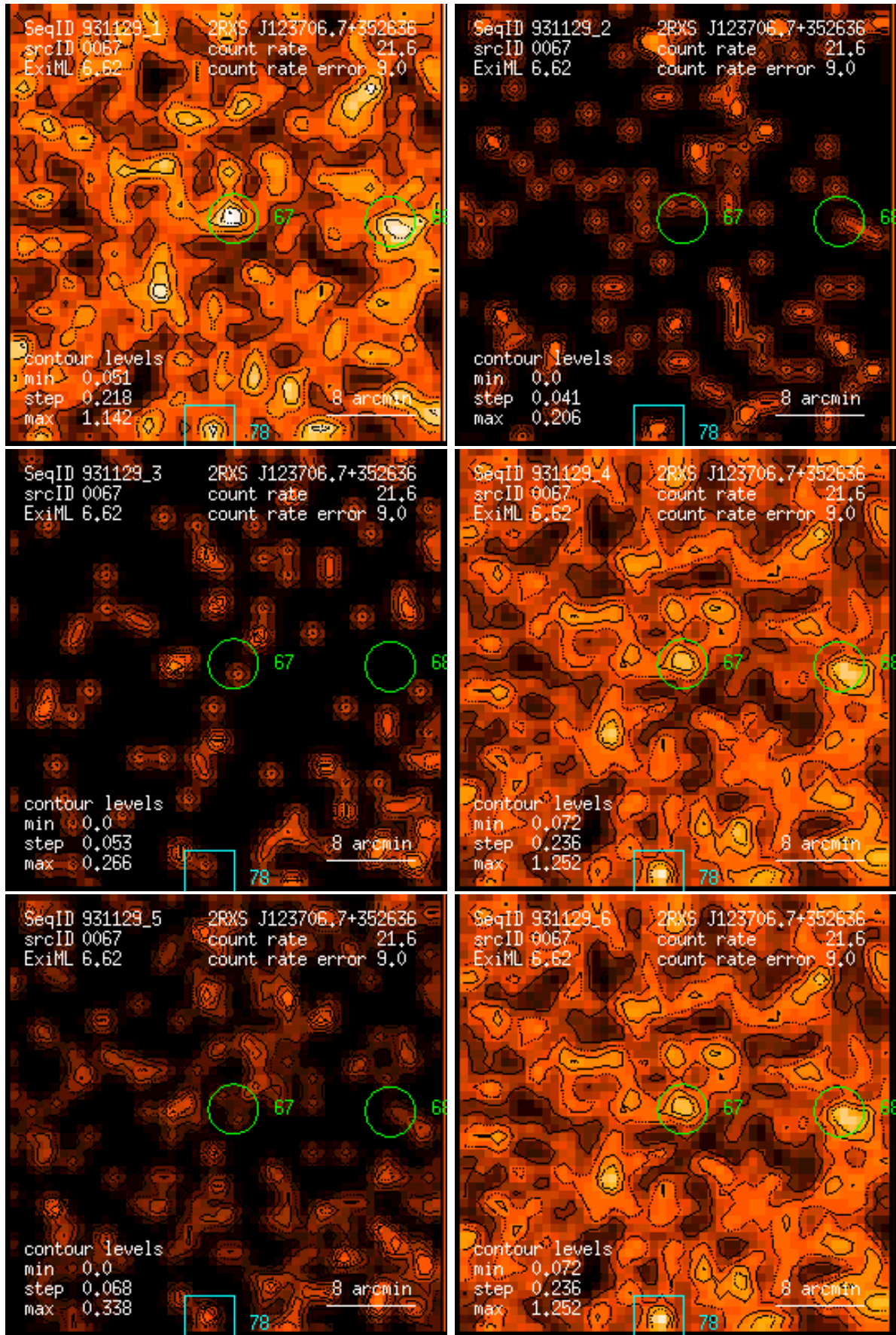
Figure 67: RASS 931129: detection 0067: band rate images, Gaussian filter: (1) PSPC channels 11 – 41, (2) 52 – 90, (3) 91 – 201, (4) 11 – 235, (5) 52 – 201, (6) 11 – 201. Broad band rates in counts/ks. Band rate contour levels in counts/ks/arcmin 2 .
