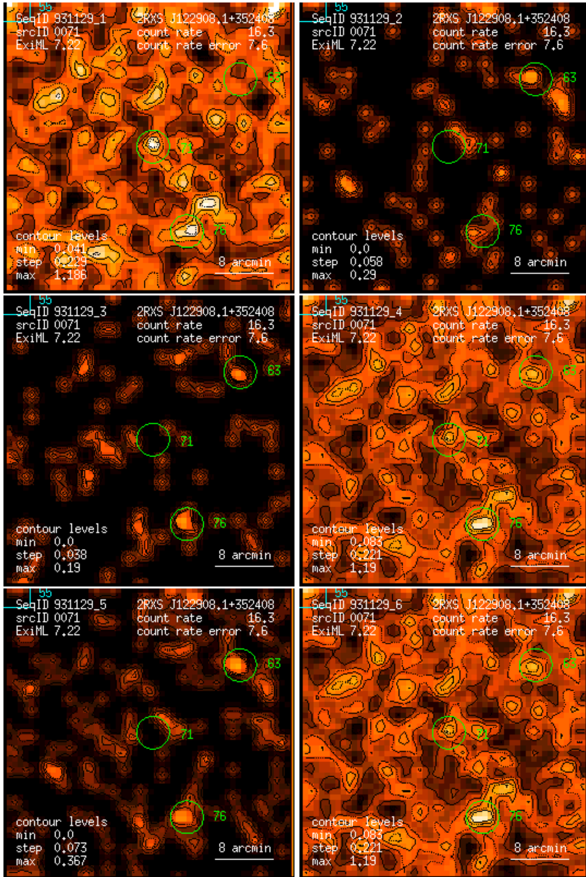
Figure 71: RASS 931129: detection 0071: band rate images, Gaussian filter: (1) PSPC channels 11 – 41, (2) 52 – 90, (3) 91 – 201, (4) 11 – 235, (5) 52 – 201, (6) 11 – 201. Broad band rates in counts/ks. Band rate contour levels in counts/ks/arcmin 2 .
