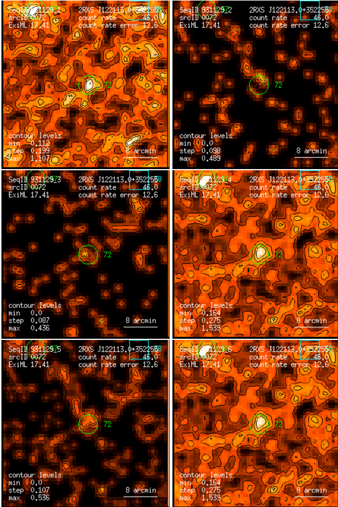
Figure 72: RASS 931129: detection 0072: band rate images, Gaussian filter: (1) PSPC channels 11 – 41, (2) 52 – 90, (3) 91 – 201, (4) 11 – 235, (5) 52 – 201, (6) 11 – 201. Broad band rates in counts/ks. Band rate contour levels in counts/ks/arcmin 2 .
