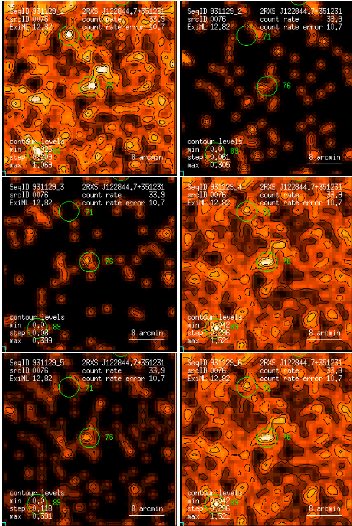
Figure 76: RASS 931129: detection 0076: band rate images, Gaussian filter: (1) PSPC channels 11 – 41, (2) 52 – 90, (3) 91 – 201, (4) 11 – 235, (5) 52 – 201, (6) 11 – 201. Broad band rates in counts/ks. Band rate contour levels in counts/ks/arcmin 2 .
