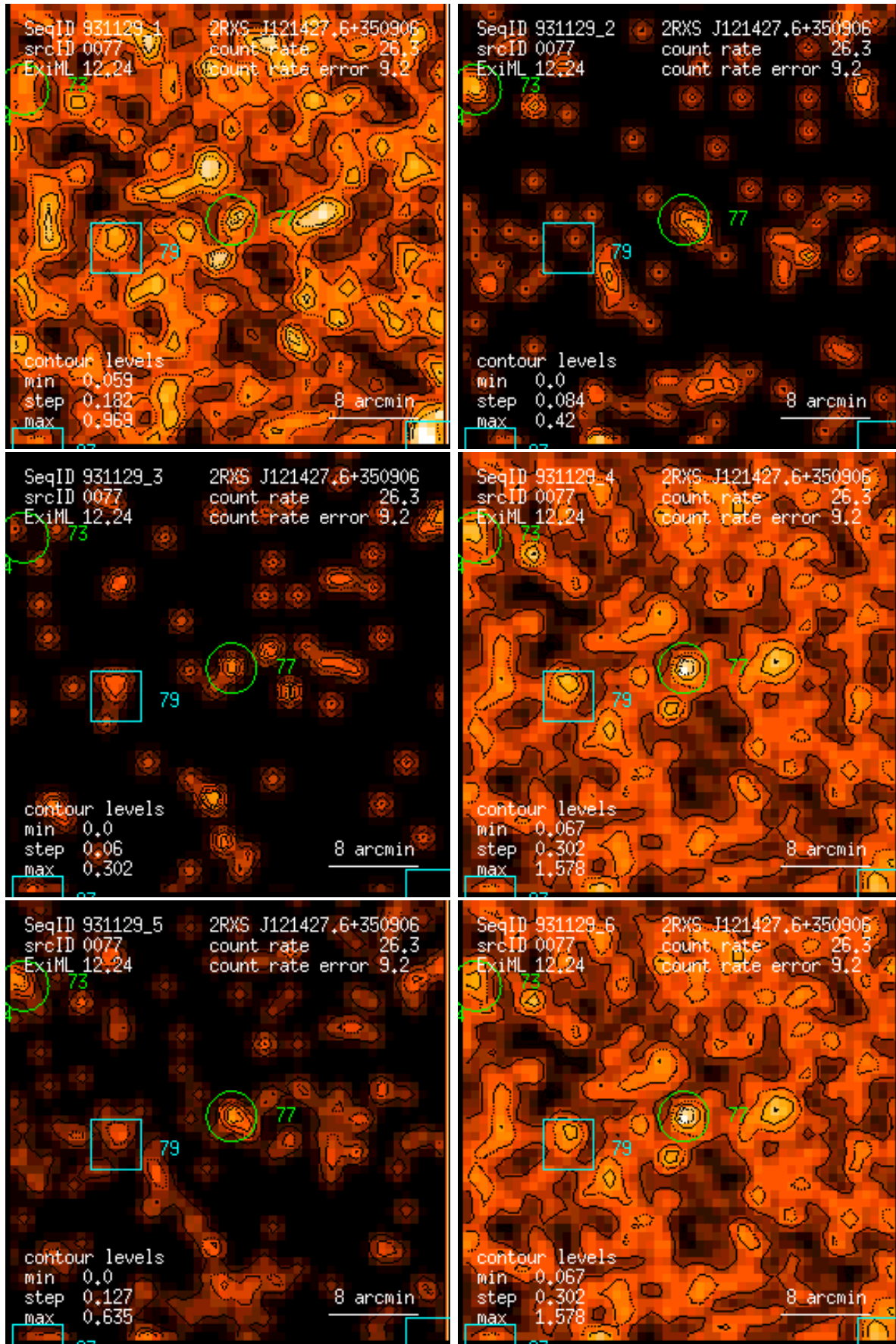
Figure 77: RASS 931129: detection 0077: band rate images, Gaussian filter: (1) PSPC channels 11 – 41, (2) 52 – 90, (3) 91 – 201, (4) 11 – 235, (5) 52 – 201, (6) 11 – 201. Broad band rates in counts/ks. Band rate contour levels in counts/ks/arcmin 2 .
