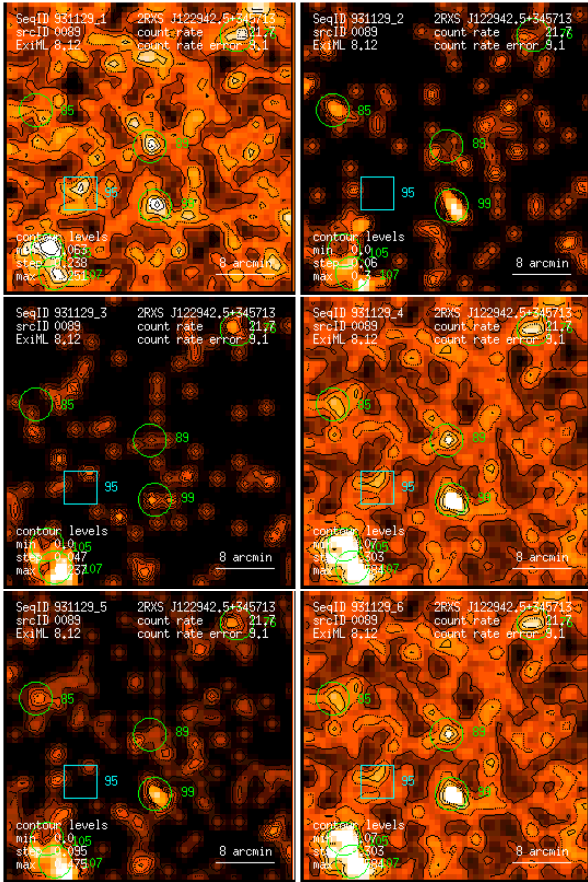
Figure 89: RASS 931129: detection 0089: band rate images, Gaussian filter: (1) PSPC channels 11 – 41, (2) 52 – 90, (3) 91 – 201, (4) 11 – 235, (5) 52 – 201, (6) 11 – 201. Broad band rates in counts/ks. Band rate contour levels in counts/ks/arcmin 2 .
