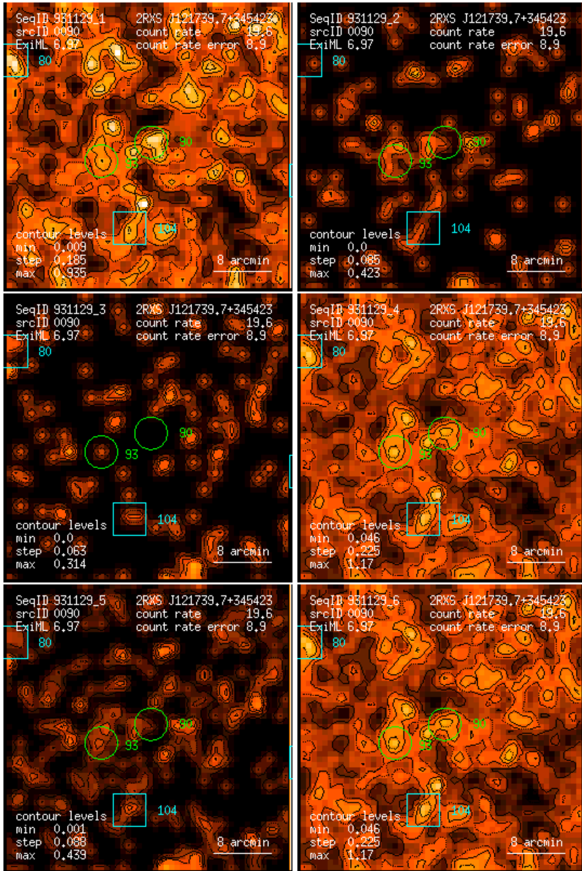
Figure 90: RASS 931129: detection 0090: band rate images, Gaussian filter: (1) PSPC channels 11 – 41, (2) 52 – 90, (3) 91 – 201, (4) 11 – 235, (5) 52 – 201, (6) 11 – 201. Broad band rates in counts/ks. Band rate contour levels in counts/ks/arcmin 2 .
